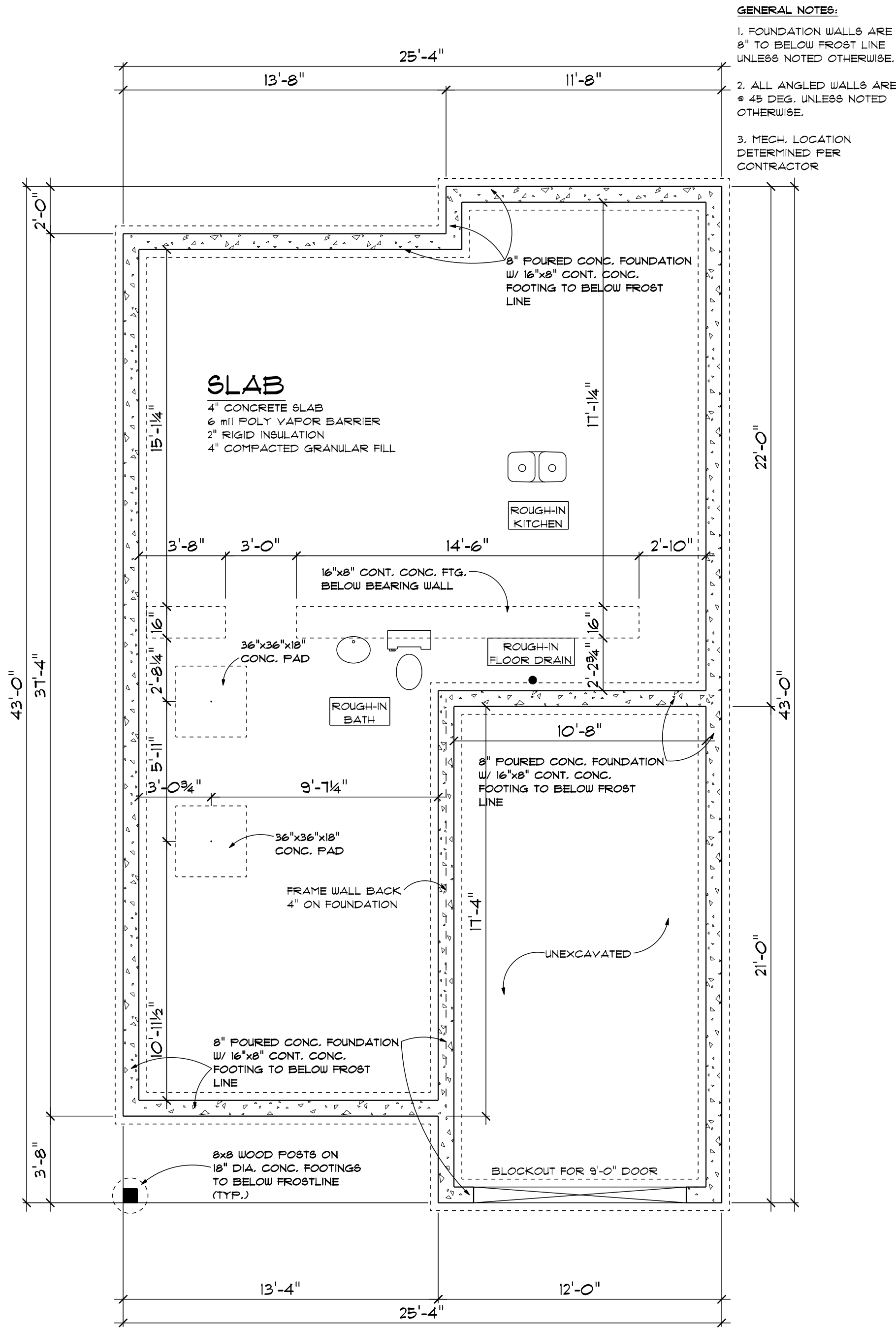
FOUNDATION PLAN
