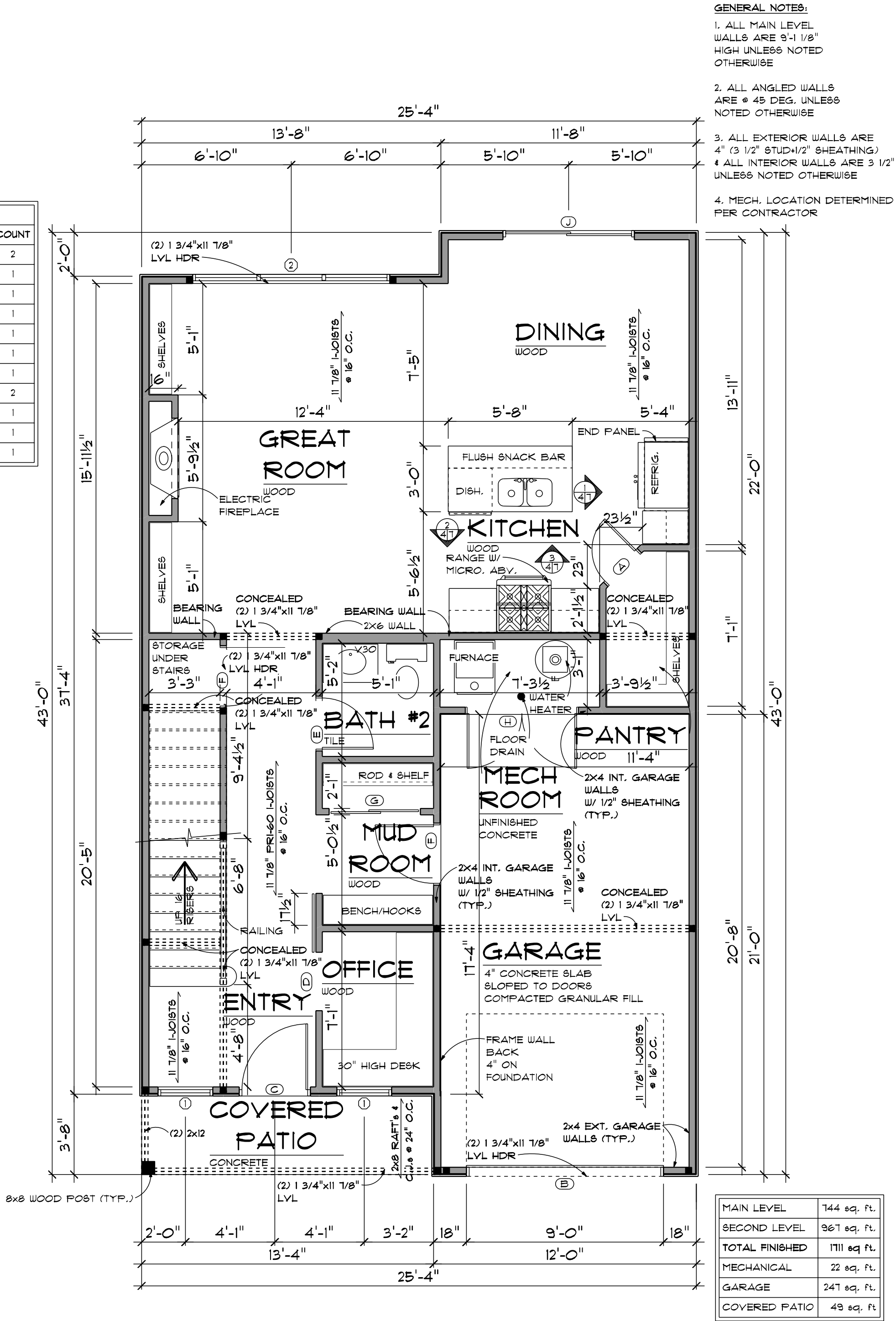
MAIN LEVEL FLOOR PLAN SCALE: 1/4" = 1'-0"
