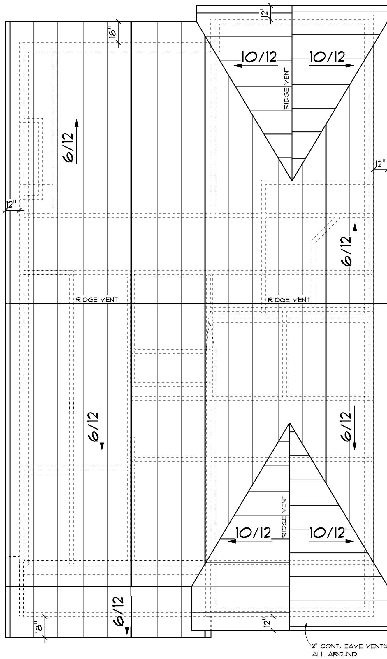
ROOF PLAN
