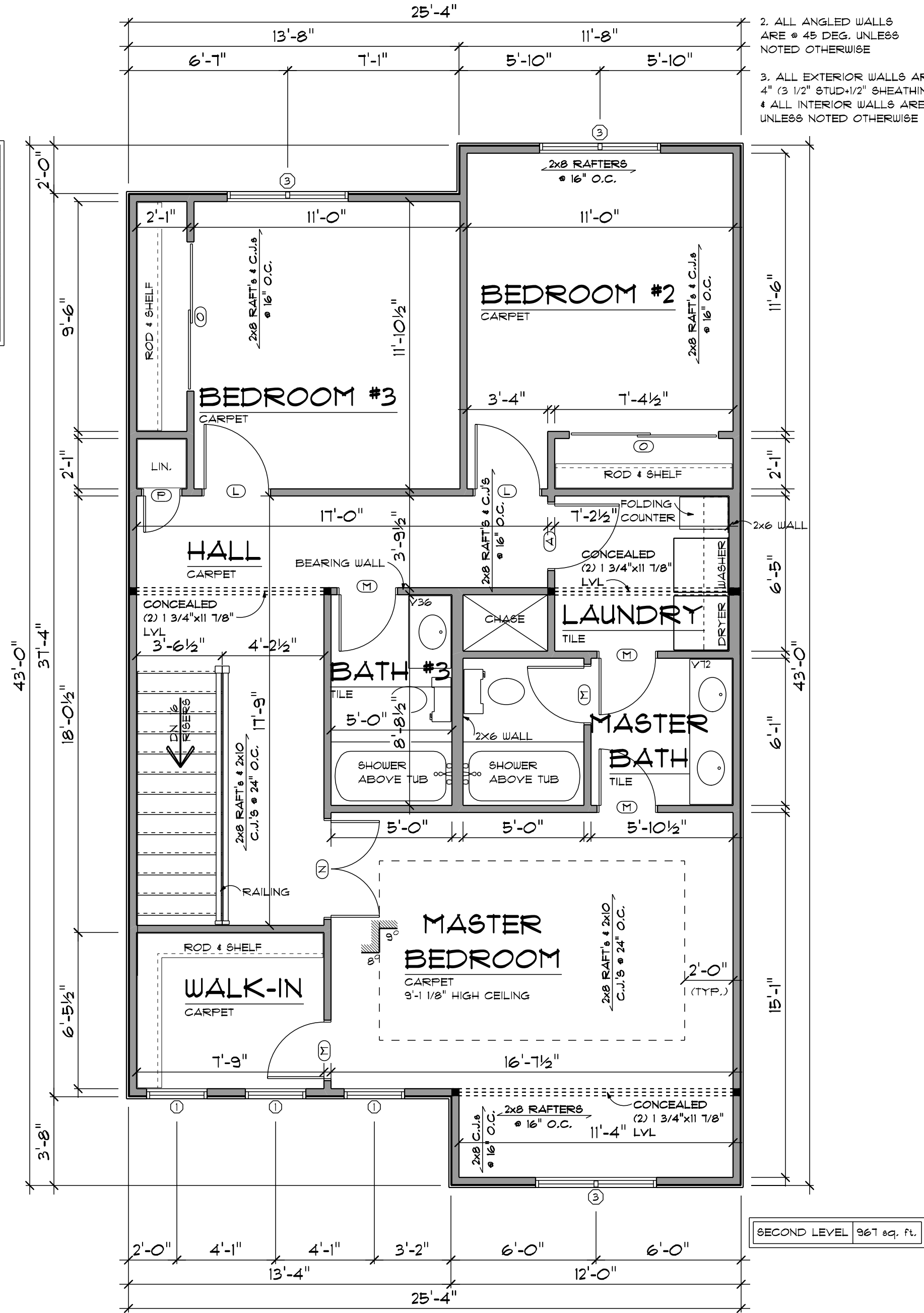
SECOND LEVEL FLOOR PLAN SCALE: 1/4" = 1'-0"
