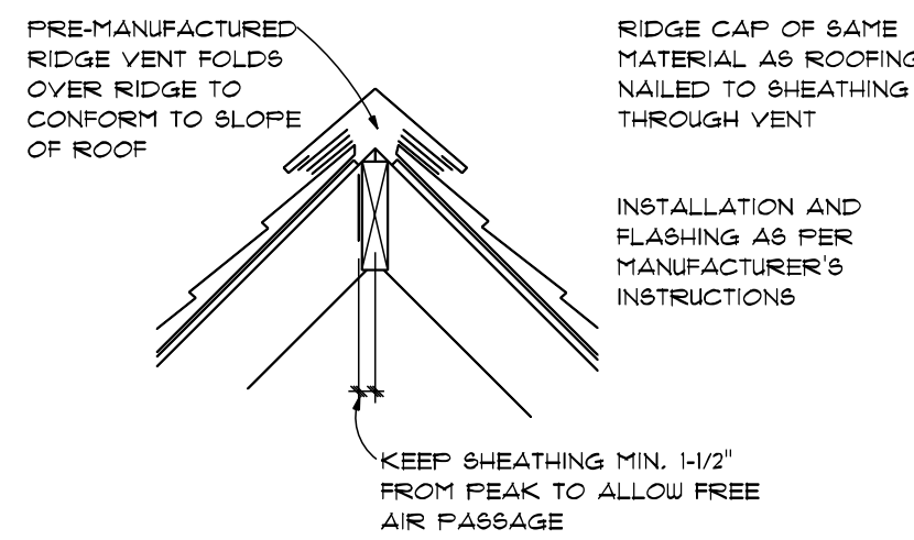
RIDGE VENT
