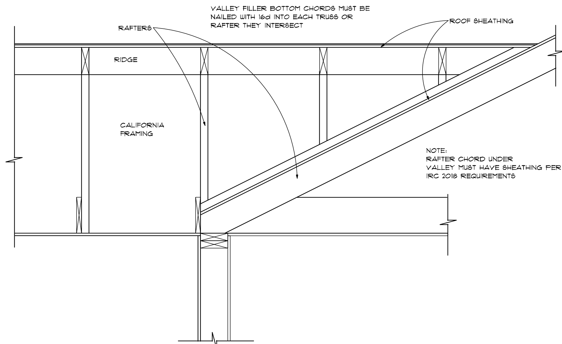
ROOF OVERFRAMING
