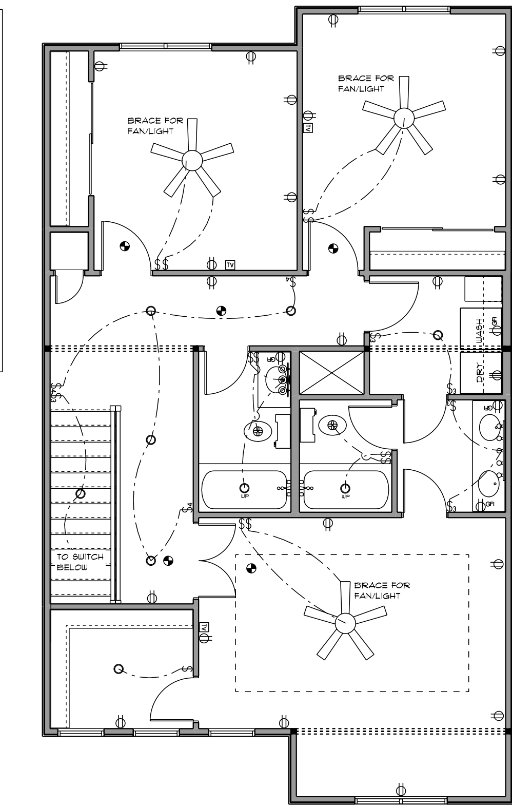
SECOND LEVEL ELECTRICAL PLAN SCALE: 3/16" = 1'-0"
