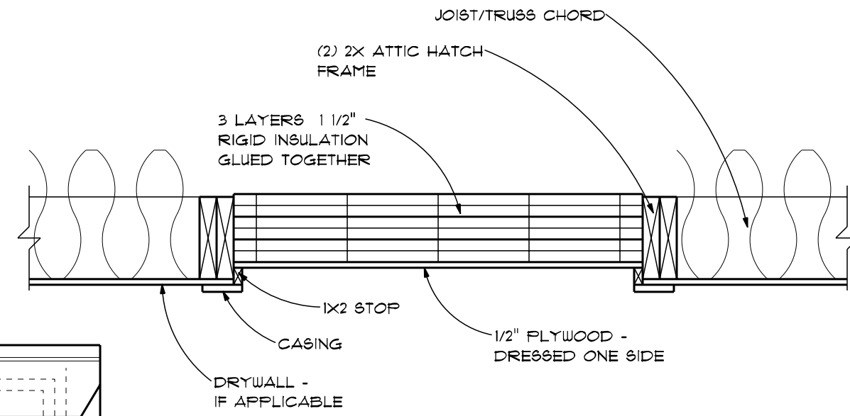
ATTIC HATCH
