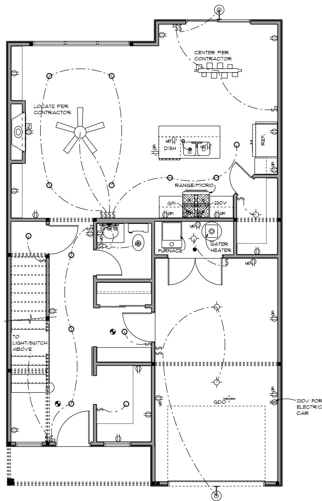
MAIN LEVEL ELECTRICAL PLAN SCALE: 3/16" = 1'-0"
