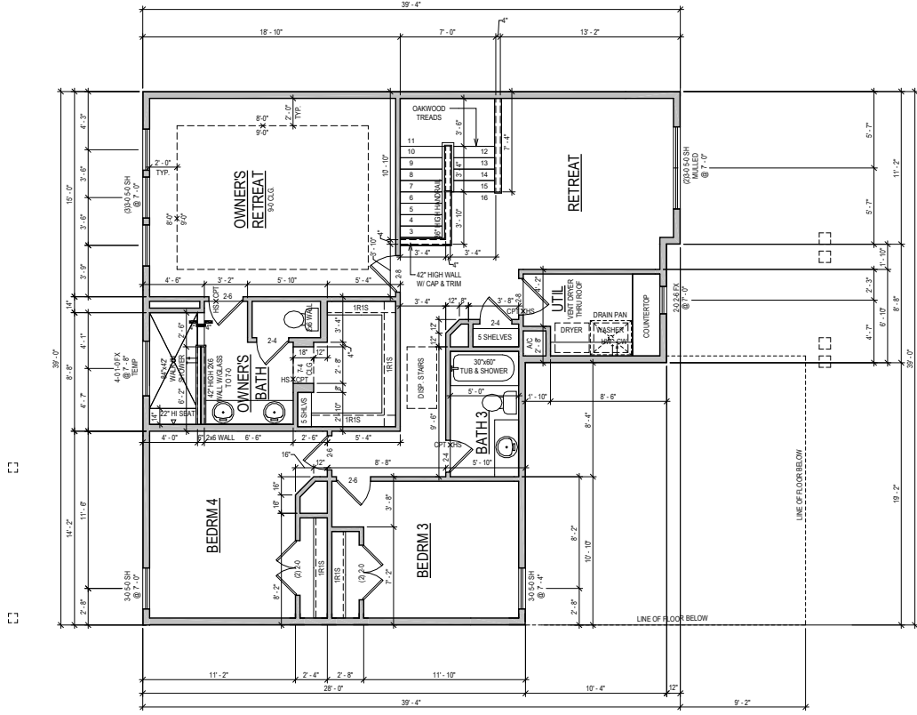
SECOND FLOOR "A"
