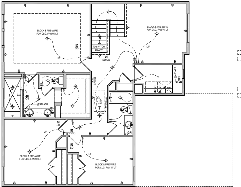
SECOND FLOOR "A"
