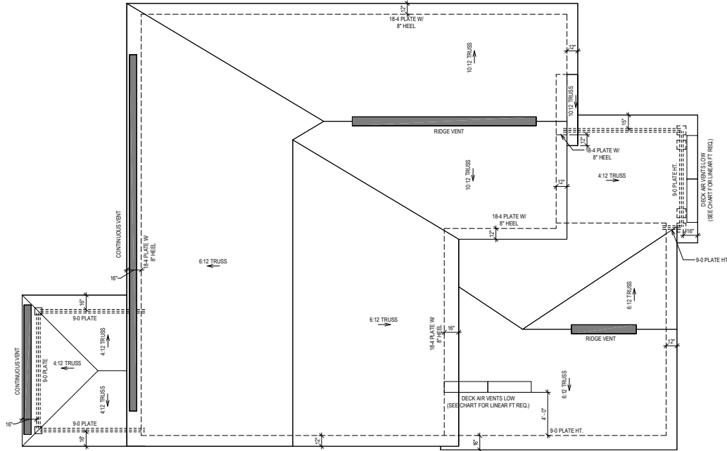
ROOF PLAN "A"
