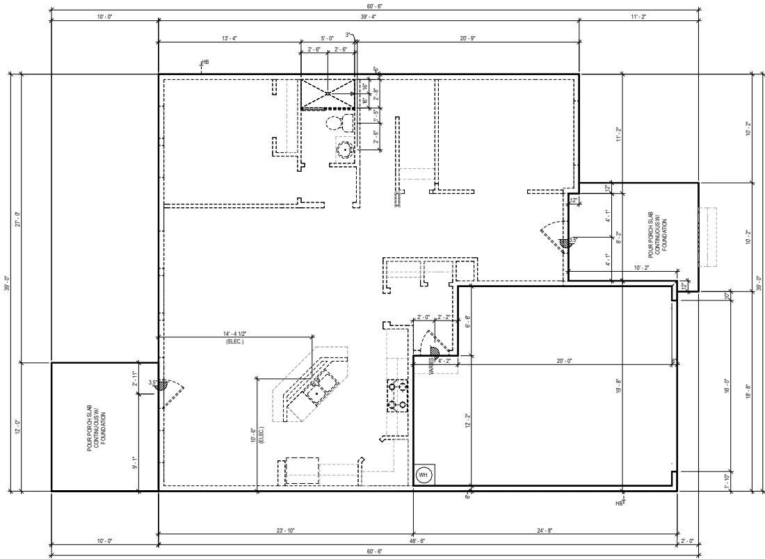
FIRST FLOOR "A"
