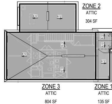
VENTILATION PLAN "A"
