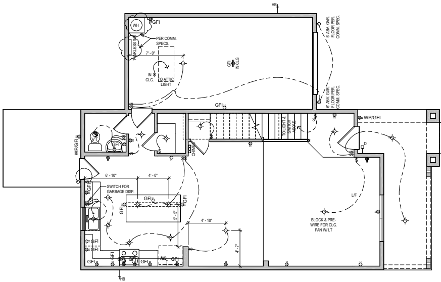
FIRST FLOOR "A"
