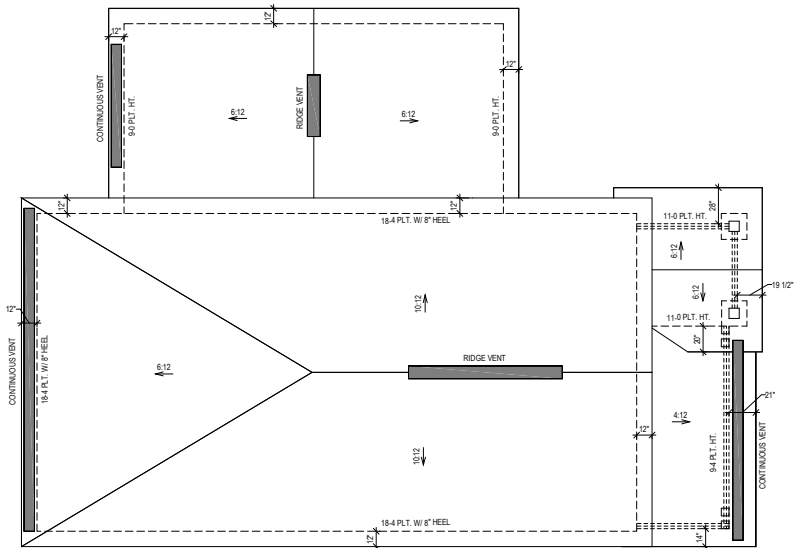
ROOF PLAN "A"
