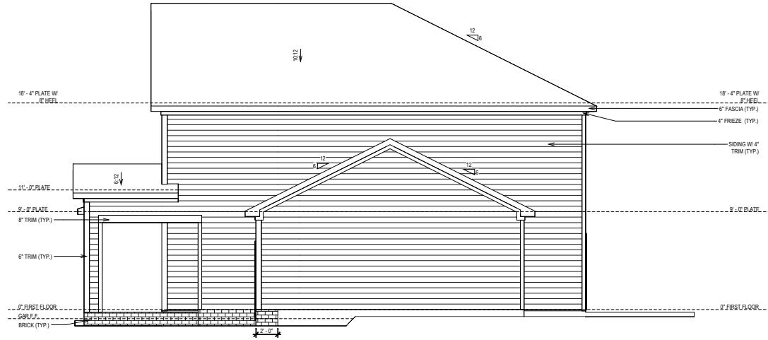
SIDE ELEVATION "A"
