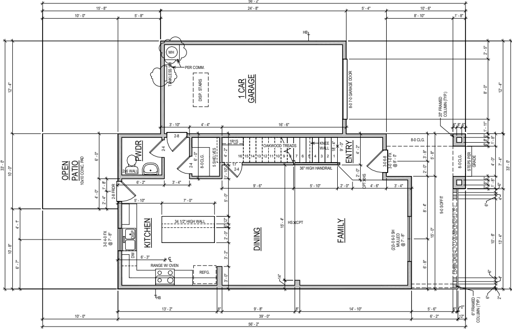
FIRST FLOOR - A"
