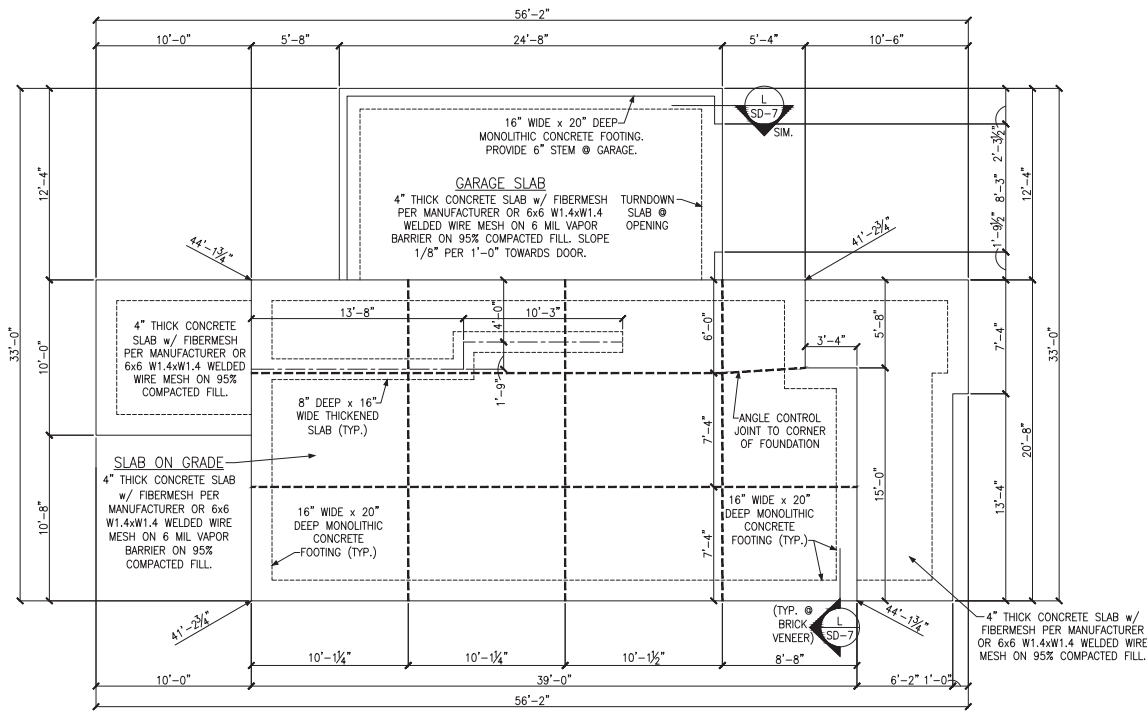
MONOLITHIC SLAB FOUNDATION PLAN
