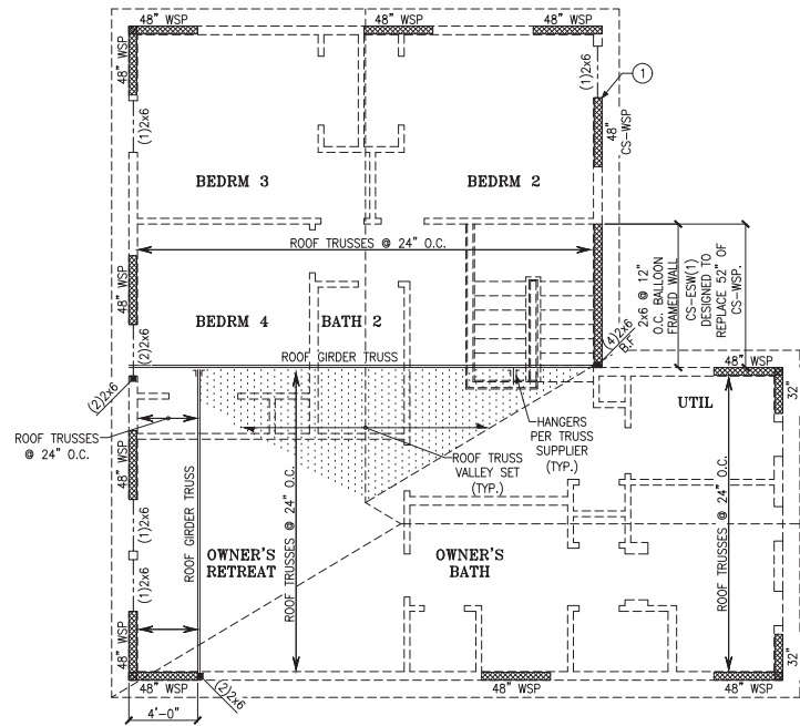
ROOF FRAMING PLAN
