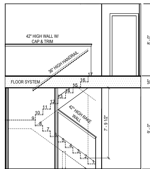
STAIR SECTION
