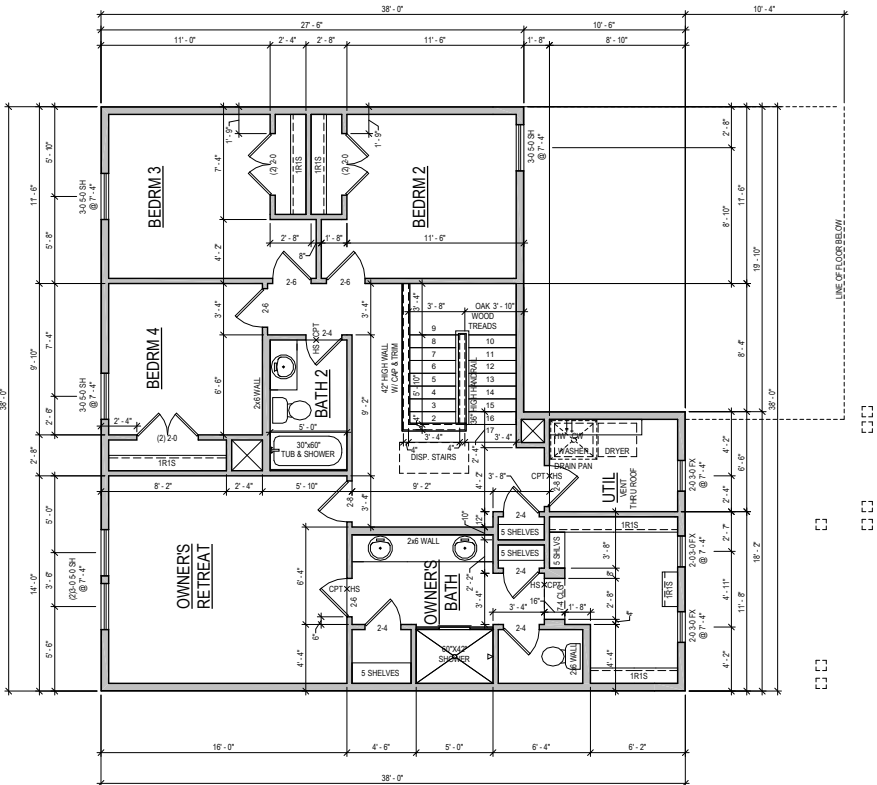
SECOND FLOOR "B"
