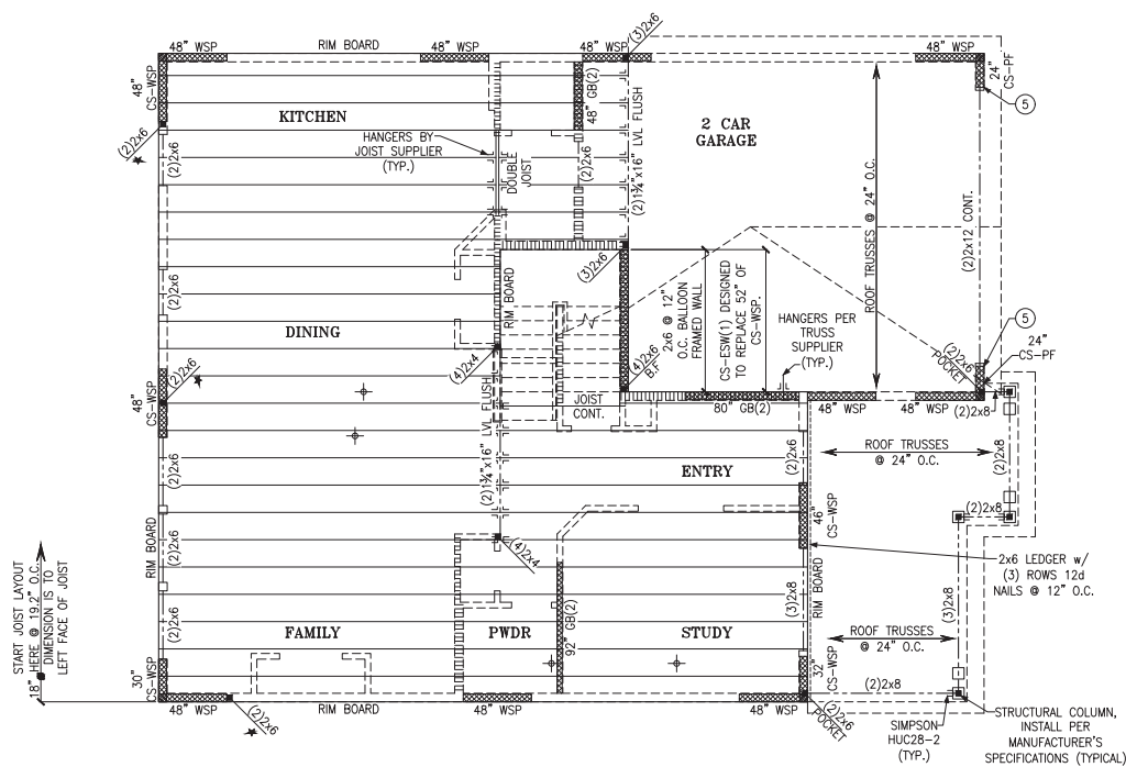
SECOND FLOOR FRAMING PLAN
