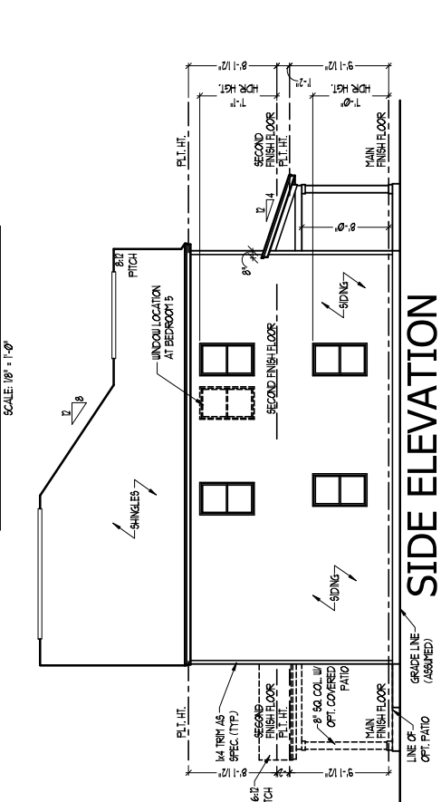
SIDE ELEVATION
