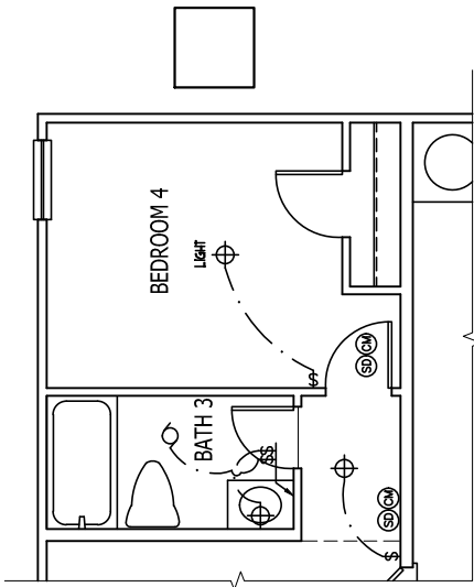
OPT BEDROOM 4 W/ BATH 3 ILO STUDY AND POWDER ROOM 1 SCALE 1/4\"/>
