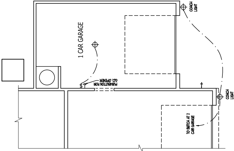
OPT 1 CAR GARAGE SCALE 1/4\"/>
