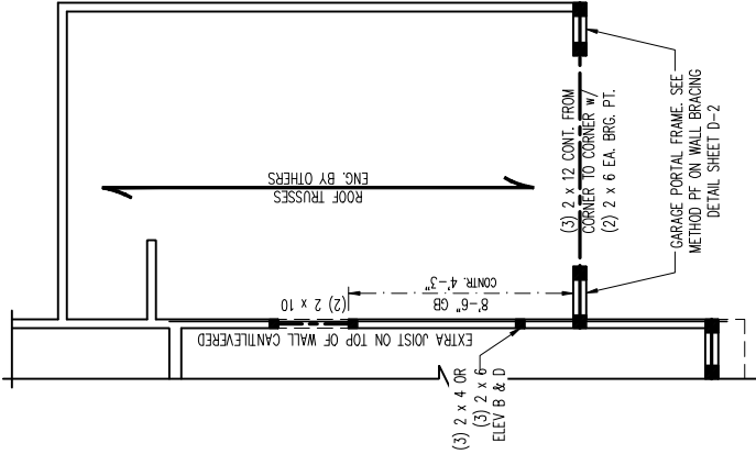
OPT. 1 CAR GARAGE
