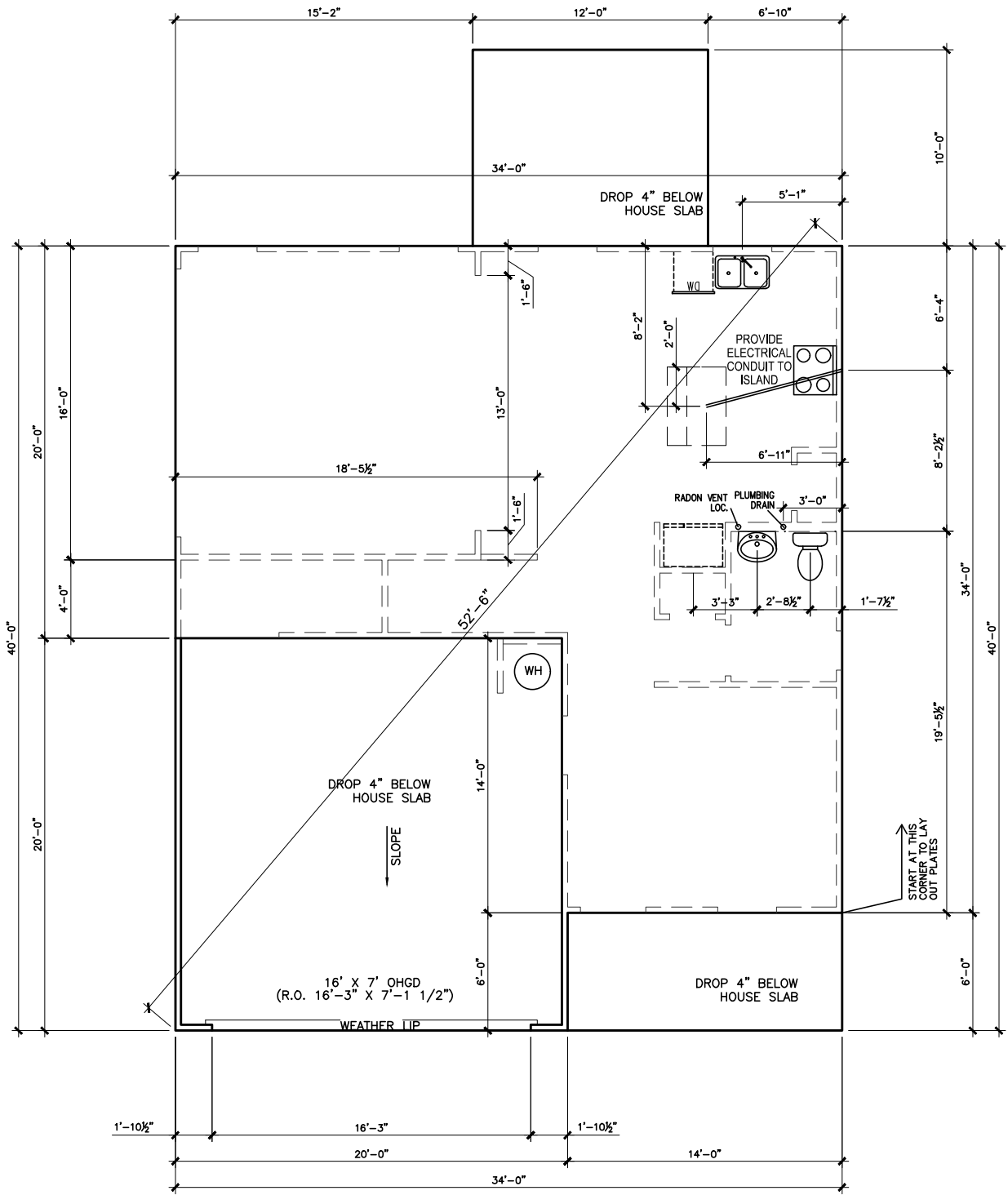
SLAB PLAN
