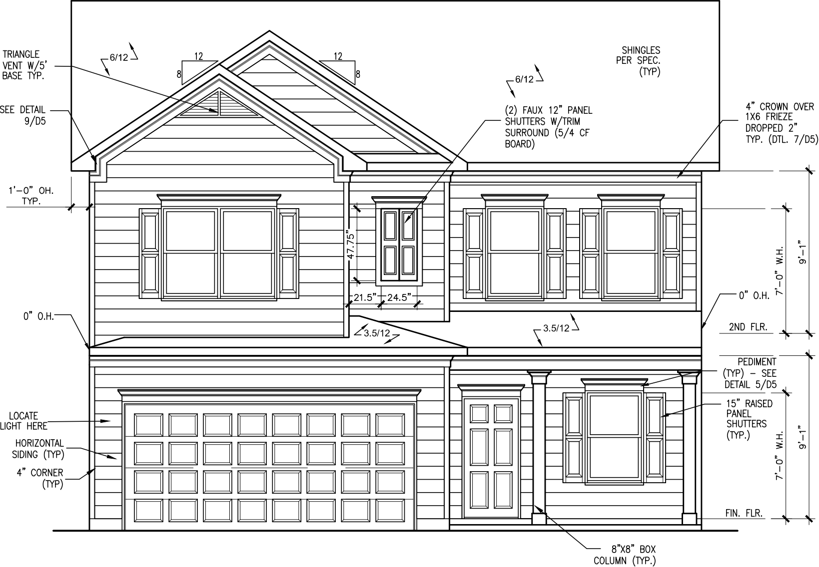
FRONT ELEVATION "A" SCALE: 3/16"=1'-0"
