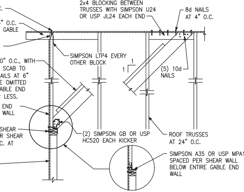
E GABLE END WALL DETAIL
