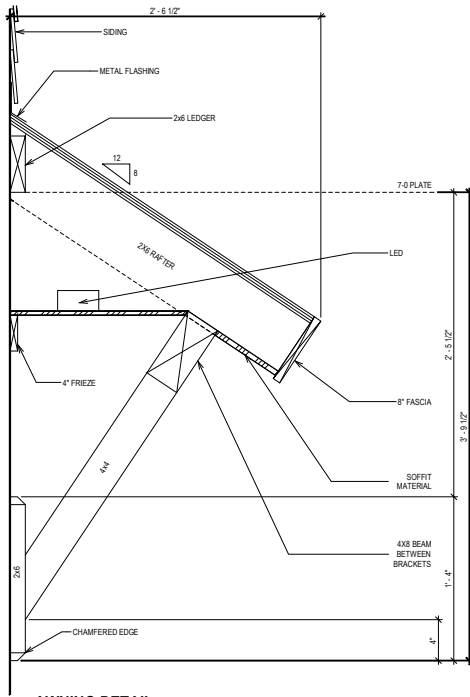
AWNING DETAIL
