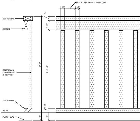
RAIL DETAIL
