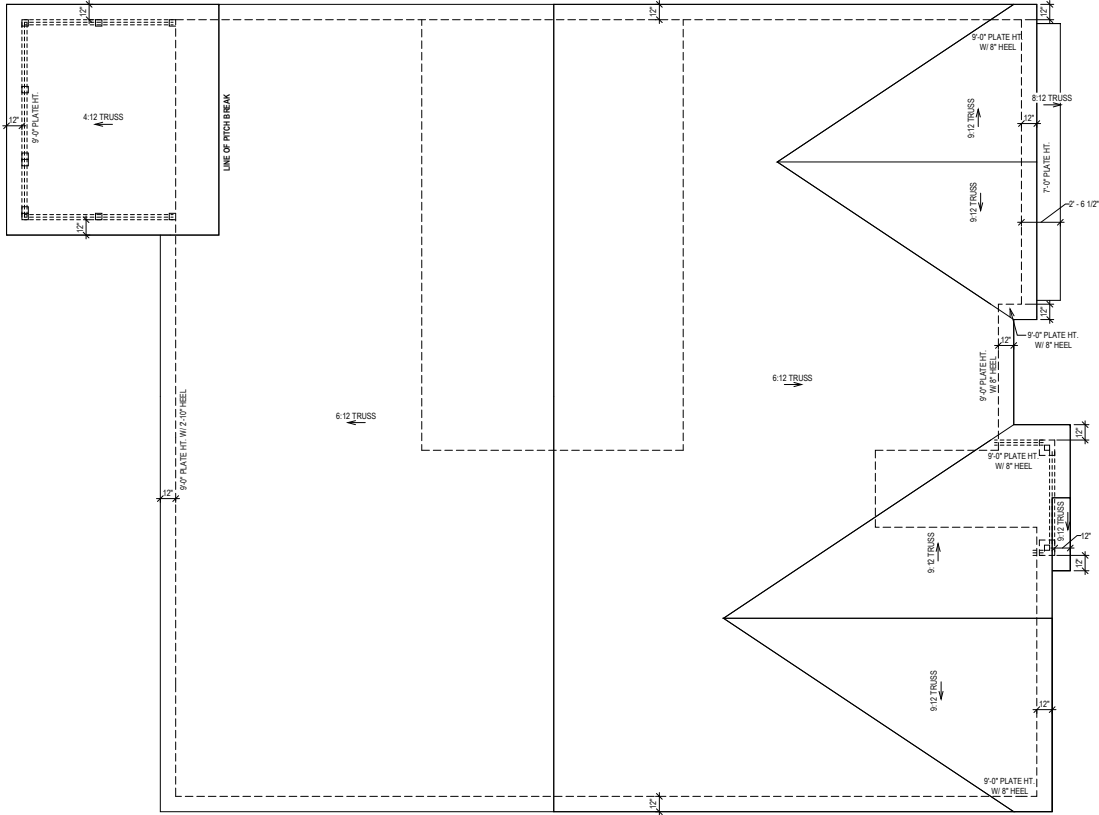
ROOF PLAN "B"
