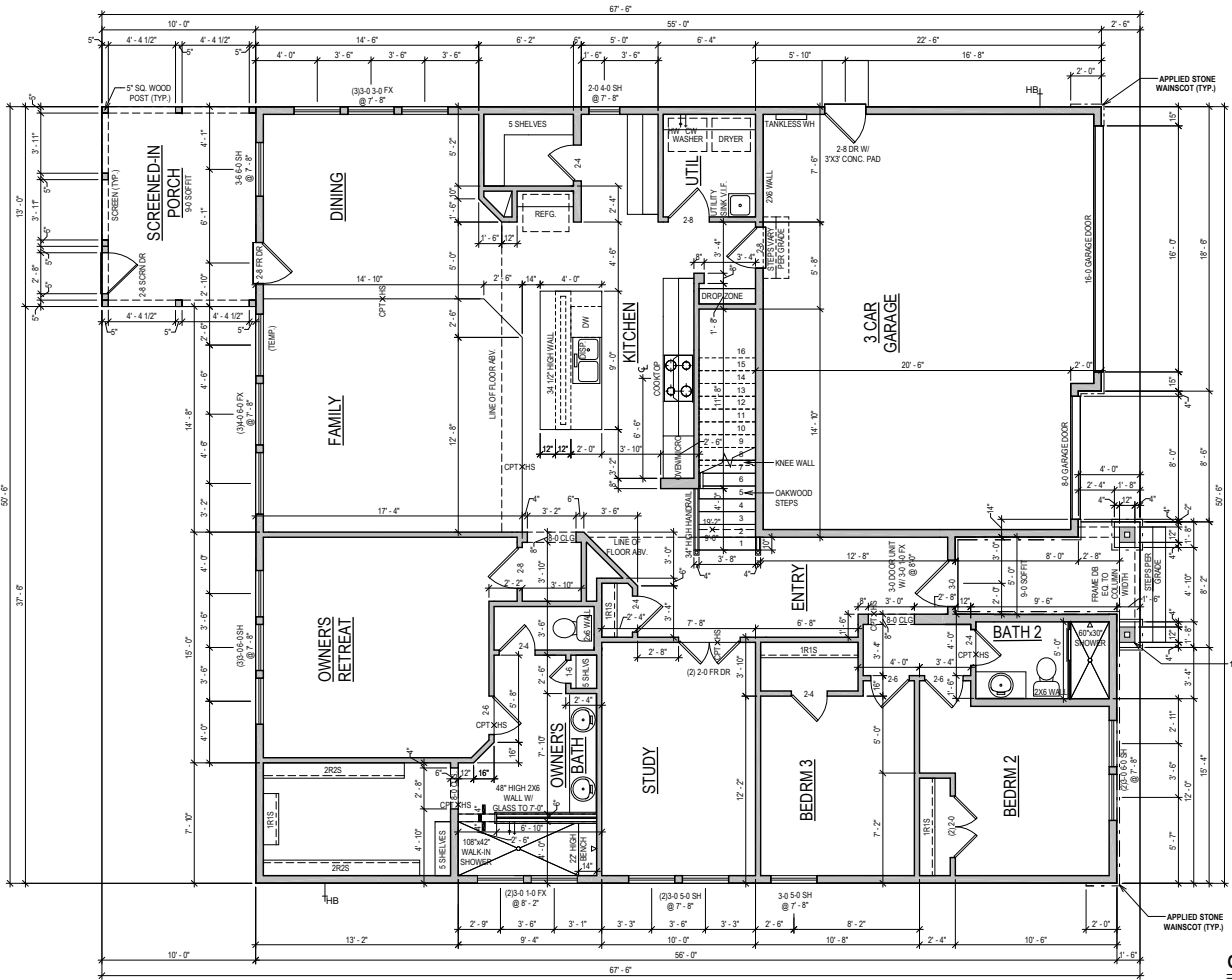
FIRST FLOOR
