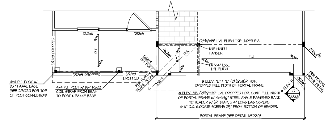
2 PARTIAL 2ND FLOOR FRAMING PLAN SCALE: 1/4"=1'-0" ON 22x34 1/8"=1'-0" ON 11x17 ELEV. B, E & H SEE ELEV. A FOR ADD'L INFO
