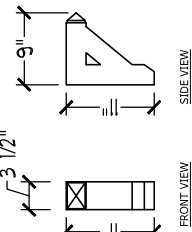
BRACKET DETAIL
