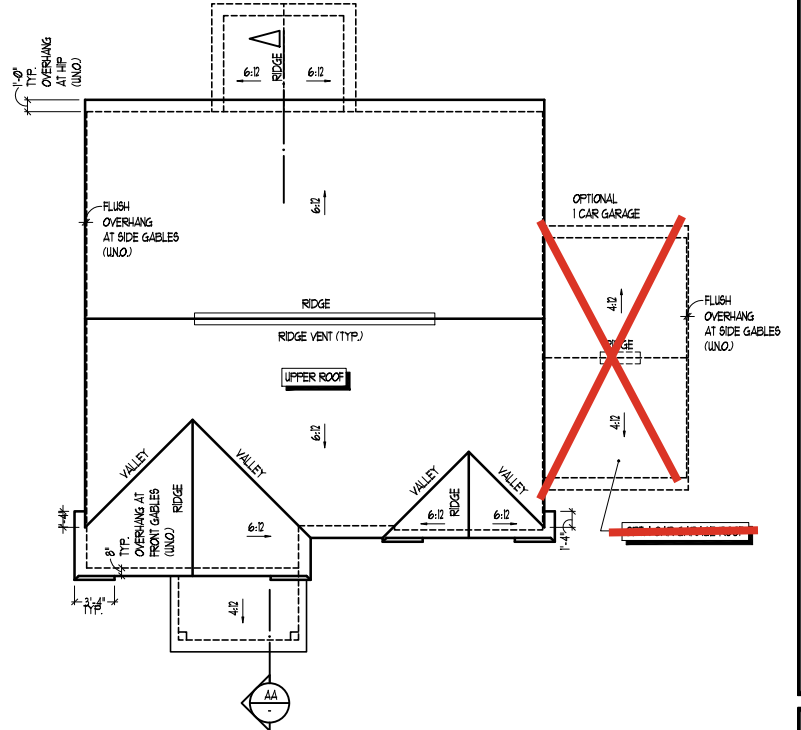
ROOF PLAN
