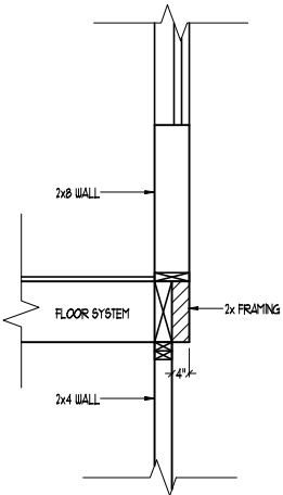
CANTILEVER DETAIL 1
