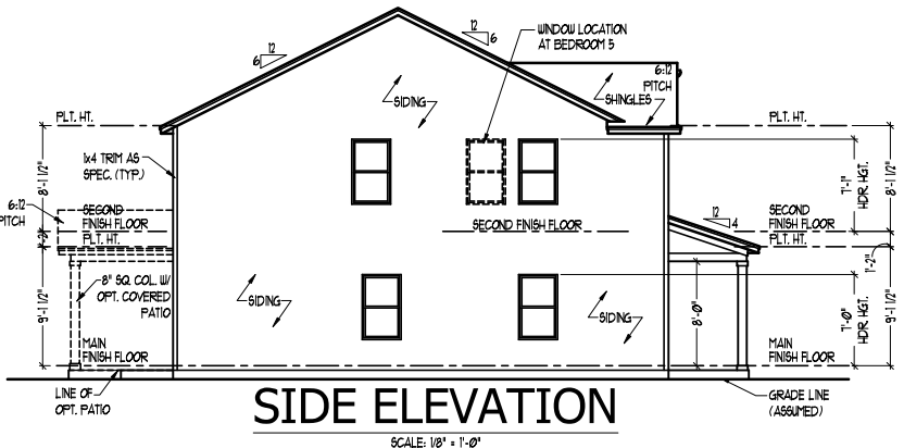
SIDE ELEVATION
