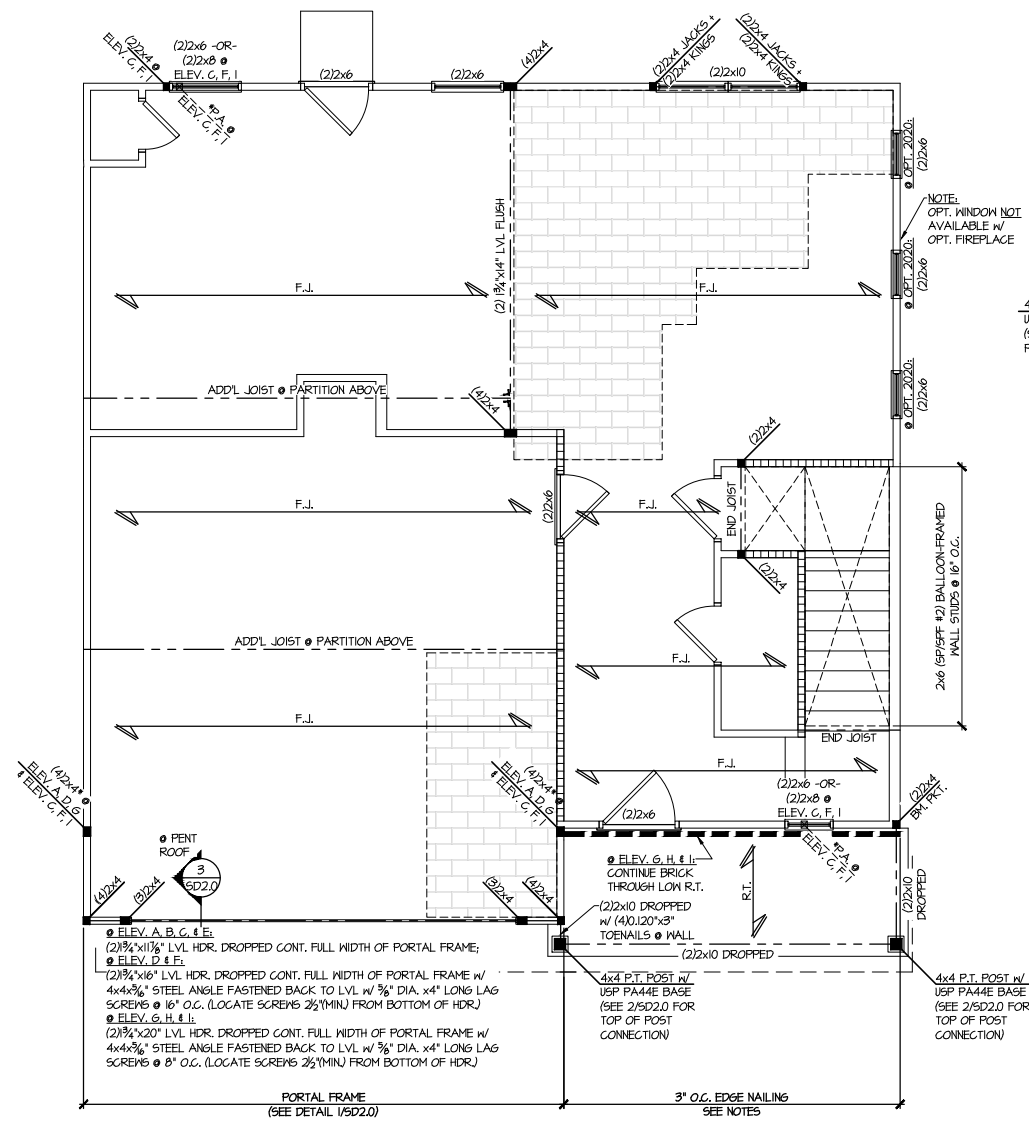
1 2ND FLOOR FRAMING PLAN SCALE: 1/4"=1'-0" ON 22x34 1/8"=1'-0" ON 11x17 ALL ELEV. SIM.
