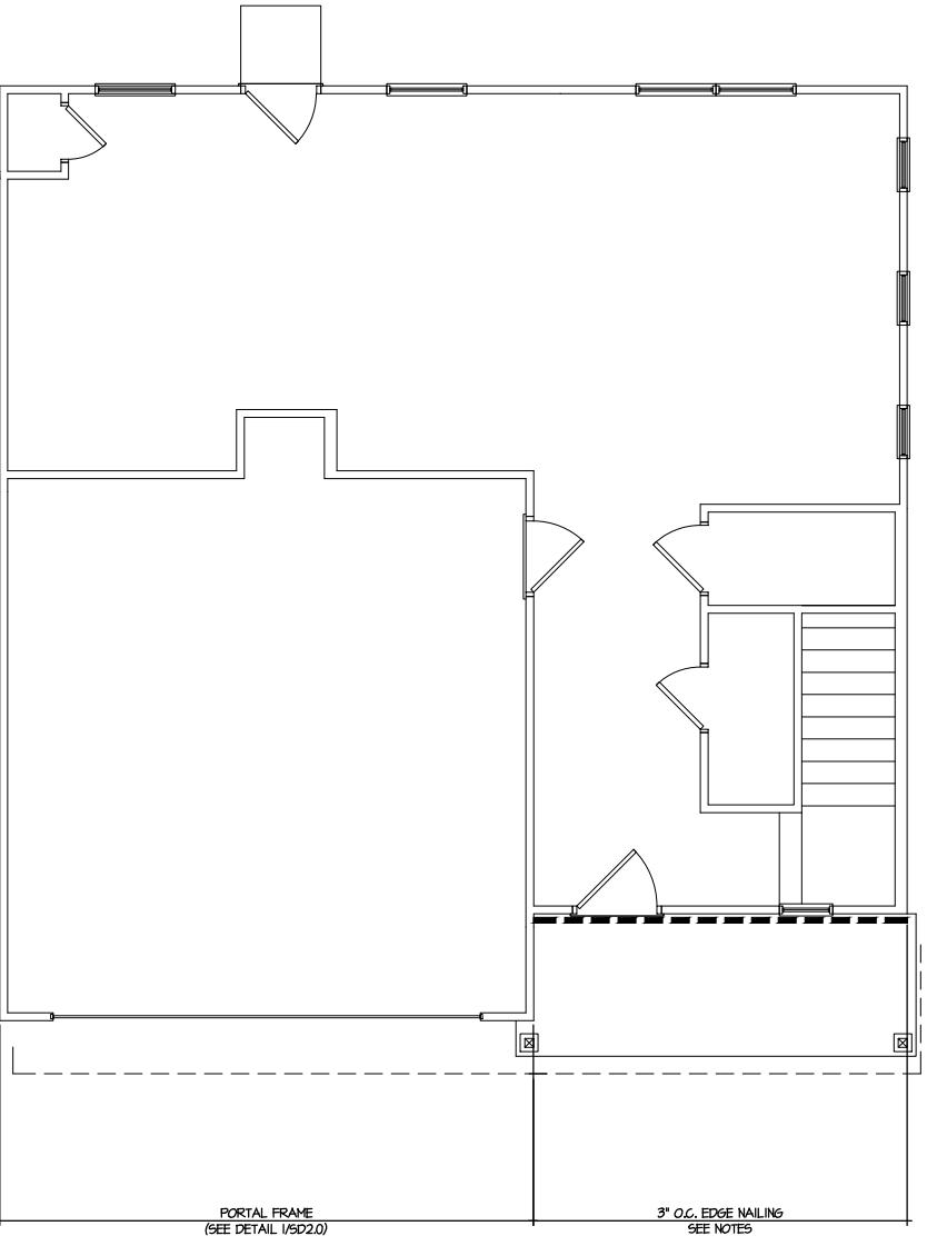
1 1ST FLOOR WALL BRACING PLAN
