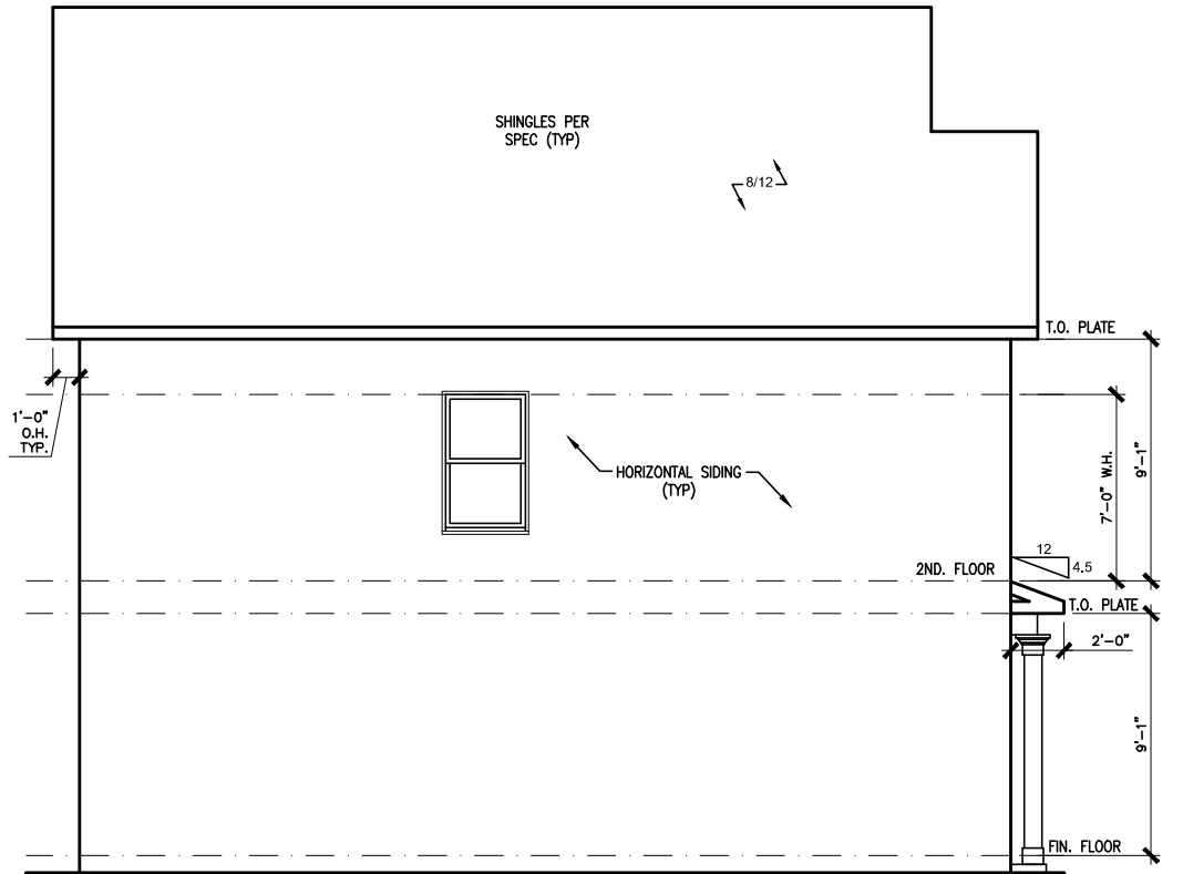
LEFT ELEVATION "B"
