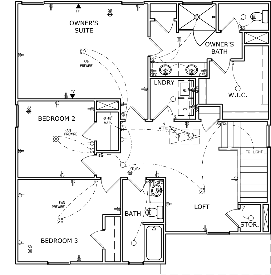
SECOND FLOOR ELECTRICAL PLAN
