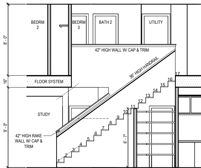
STAIR SECTION
