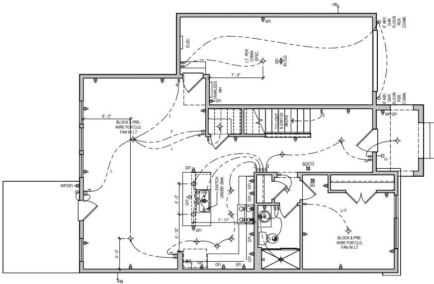
FIRST FLOOR "C"
