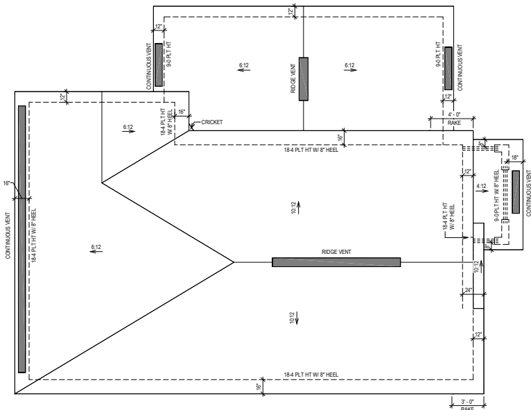
ROOF PLAN "C"
