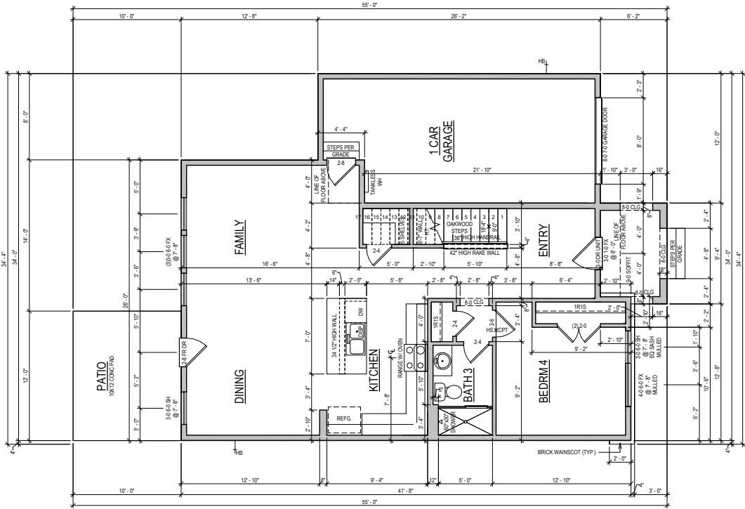
FIRST FLOOR "C"
