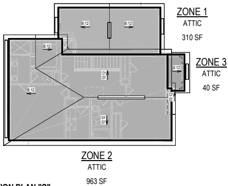
VENTILATION PLAN "C"
