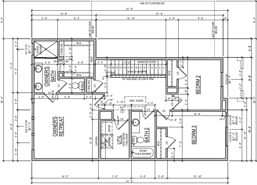
SECOND FLOOR "C"
