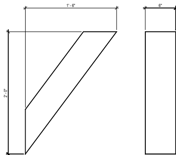
BRACKET DETAIL - BKTS18X24X6S
