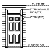
ENTRY DETAIL "B"
