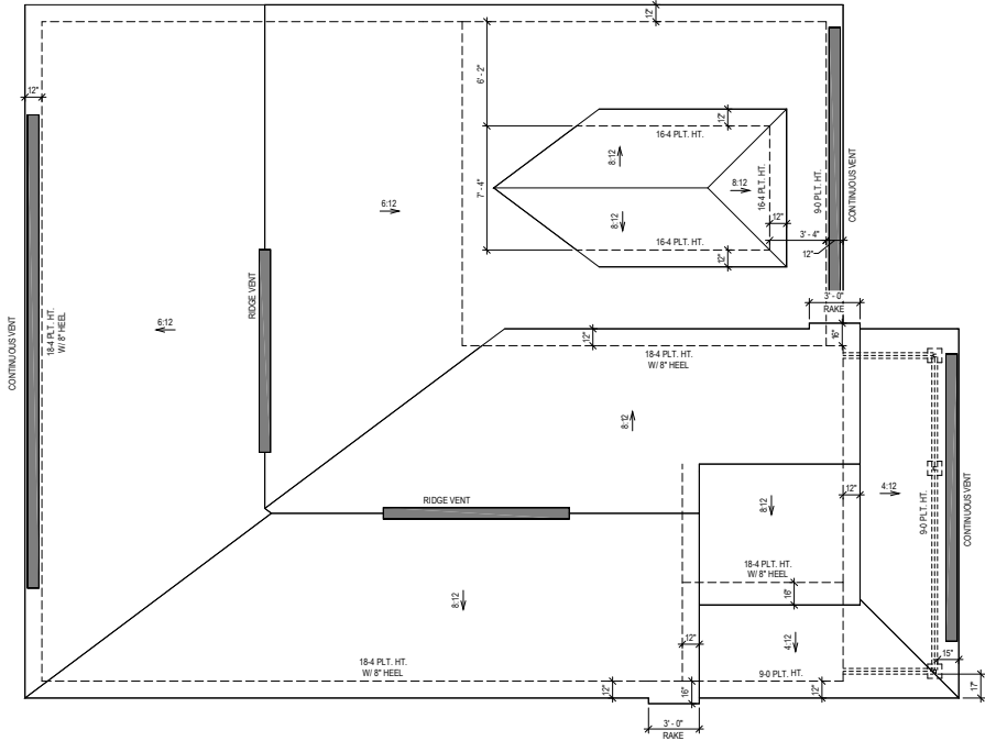
ROOF PLAN "B"
