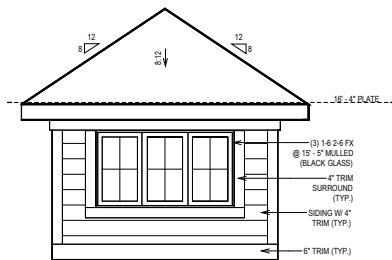
DORMER DETAIL "B"
