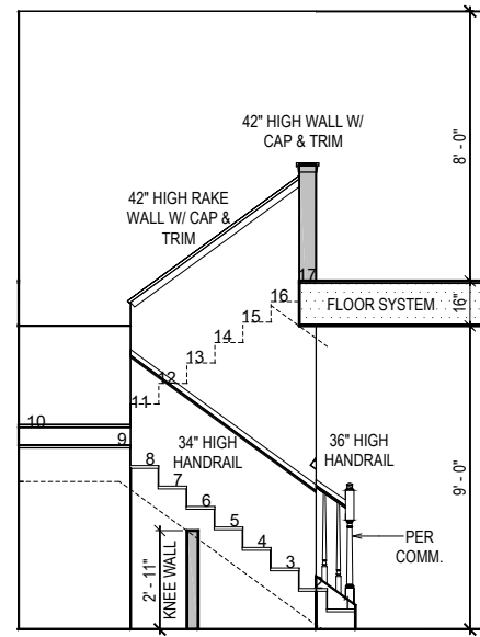
STAIR SECTION
