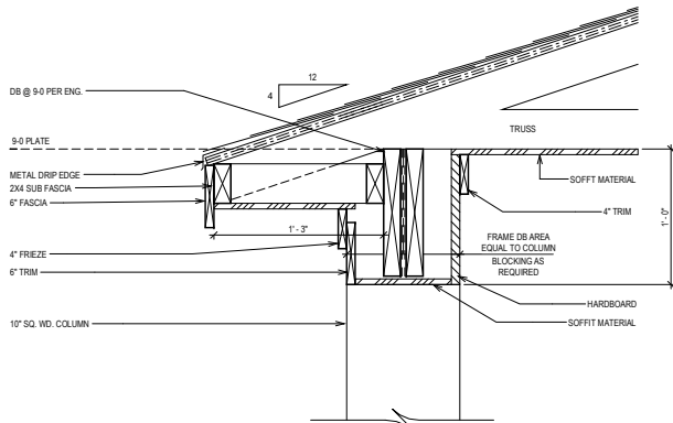
DTL - CORNICE DETAIL "B"
