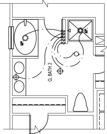
OPT OWNER'S BATH 2 SCALE 1/4" = 1'-0"
