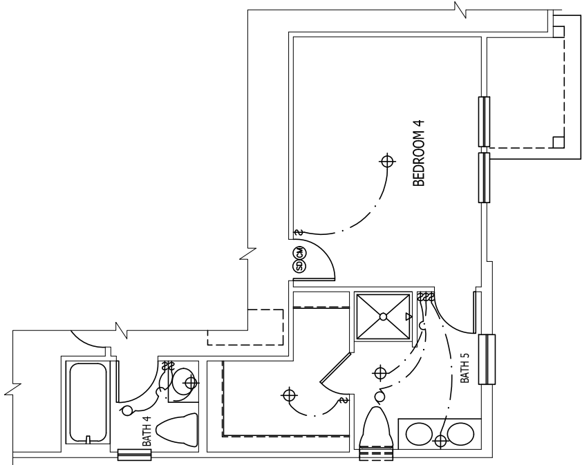
OPT BEDROOM 4/ BATH 5 ILO BEROOM 3 AND OFFICE SCALE 1/4" = 1'-0"
