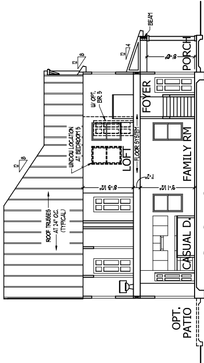
SECTION AA
