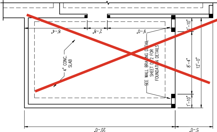
OPTIONAL 1 CAR GARAGE
