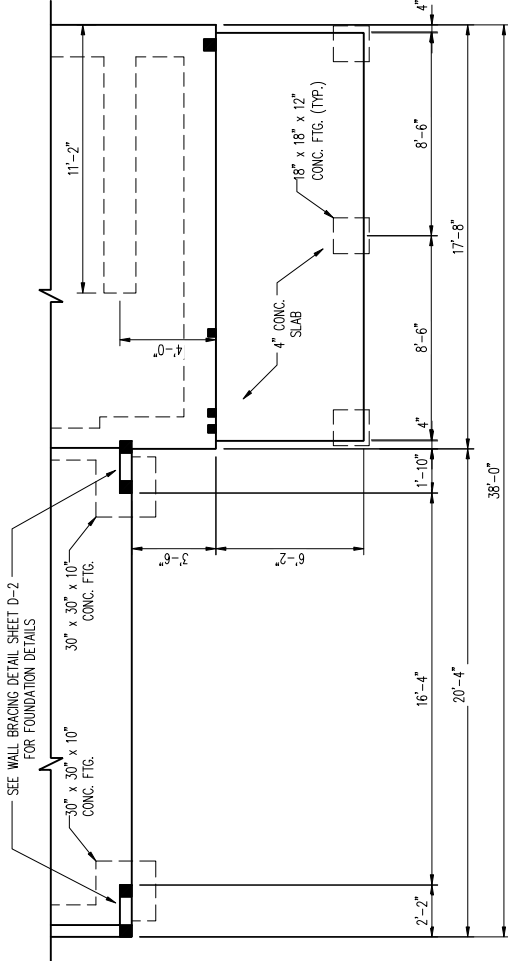
ELEVATION D
