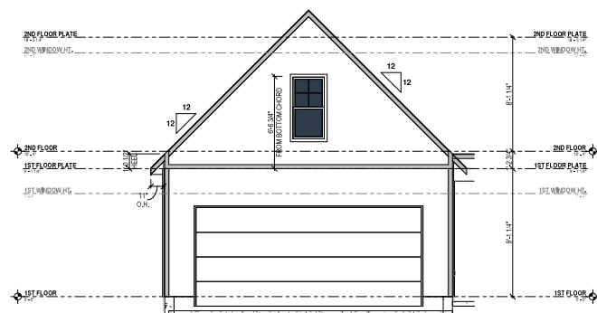
1 GARAGE A
