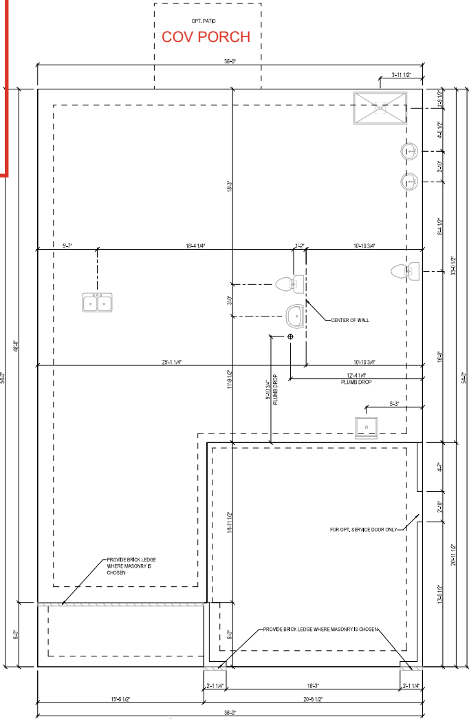
1 Mono Slab - A A-4.1 1/8" = 1'-0" 1/4" = 1'-0" WHEN PRINTED ON 11"x17" / ANSI B PAPER SIZE WHEN PRINTED ON 22"x34" / ANSI D PAPER SIZE
