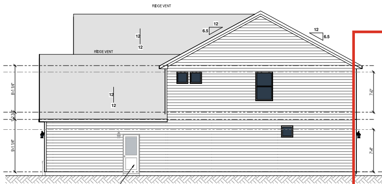
4 RIGHT ELEVATION - A A-1.1 3/32" = 1'-0" WHEN PRINTED ON 11"x17" / ANSI B PAPER SIZE 1/4" = 1'-0" WHEN PRINTED ON 22"x34" / ANSI D PAPER SIZE
