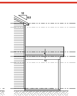
6 RIGHT - Cov'd Porch A A-1.1 3/32" = 1'-0" WHEN PRINTED ON 11"x17" / ANSI B PAPER SIZE 1/4" = 1'-0" WHEN PRINTED ON 22"x34" / ANSI D PAPER SIZE
