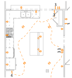
3 Opt. Gourmet Kitchen A-6 1/8" = 1'-0" WHEN PRINTED ON 11"x17" / ANSI B PAPER SIZE 1/4" = 1'-0" WHEN PRINTED ON 22"x34" / ANSI D PAPER SIZE
