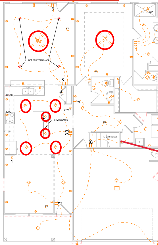
4 Opt. Cov'd Porch Elec A-6 1/8" = 1'-0" WHEN PRINTED ON 11"x17" / ANSI B PAPER SIZE 1/4" = 1'-0" WHEN PRINTED ON 22"x34" / ANSI D PAPER SIZE
