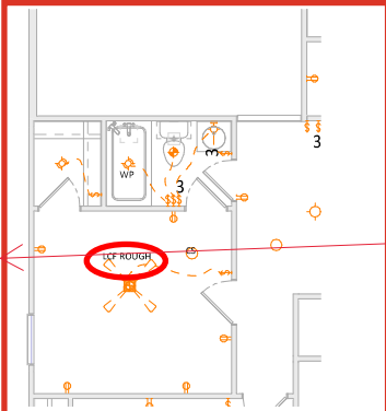
3 Opt. Bed 5 No Rec Elec A-7 1/8" = 1'-0" WHEN PRINTED ON 11"x17" / ANSI B PAPER SIZE 1/4" = 1'-0" WHEN PRINTED ON 22"x34" / ANSI D PAPER SIZE
