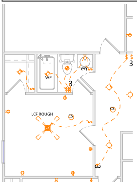
4 Opt. Bed 5 w Rec Elec A-7 1/8" = 1'-0" WHEN PRINTED ON 11"x17" / ANSI B PAPER SIZE 1/4" = 1'-0" WHEN PRINTED ON 22"x34" / ANSI D PAPER SIZE
