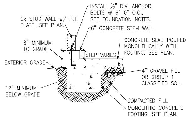
FOUNDATION SECTION EXTERIOR GARAGE WALL
