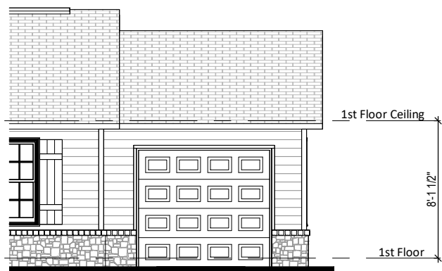
④ Front Elevation - Elev 2 Opt 1Car Garage 1/8" = 1'-0"
