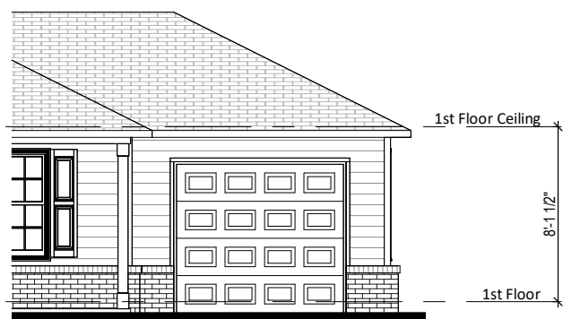
⑩ Front Elevation - Elev 4 Opt 1Car Garage 1/8" = 1'-0"
