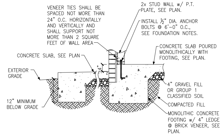
FOUNDATION SECTION EXTERIOR WALL AT PORCH w/ BRICK VENEER
