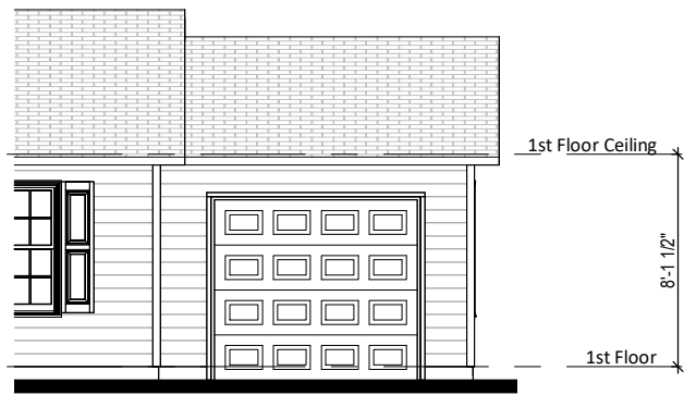
① Front Elevation - Elev 1 Opt 1Car Garage 1/8" = 1'-0"
