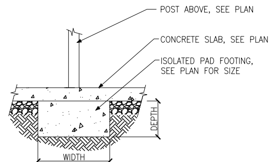
ISOLATED PAD FOOTING INTERIOR COLUMN
