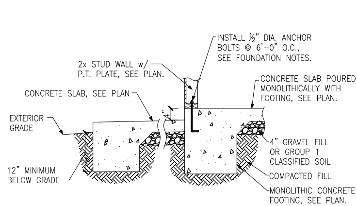
© FOUNDATION SECTION EXTERIOR WALL AT PORCH
