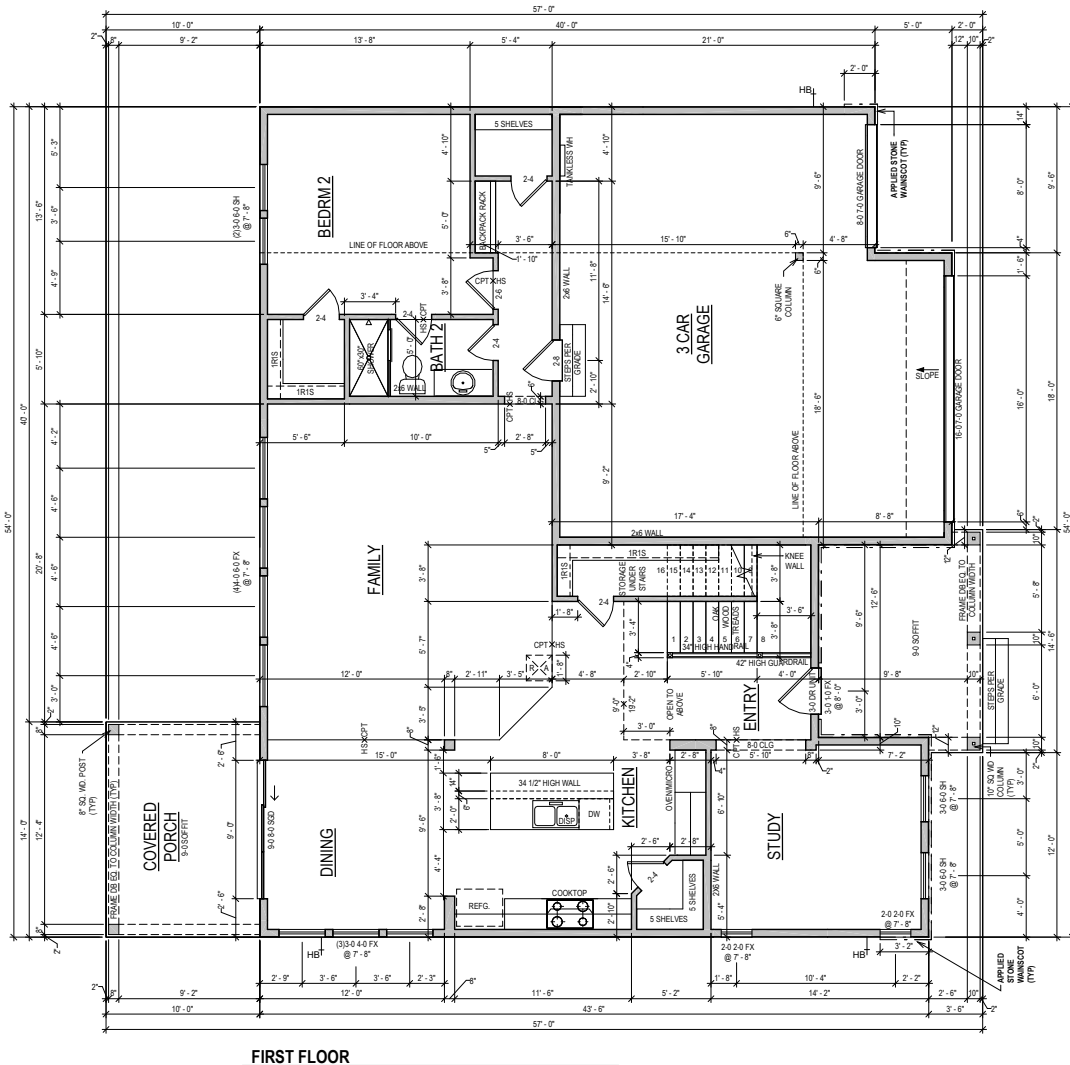
FIRST FLOOR
