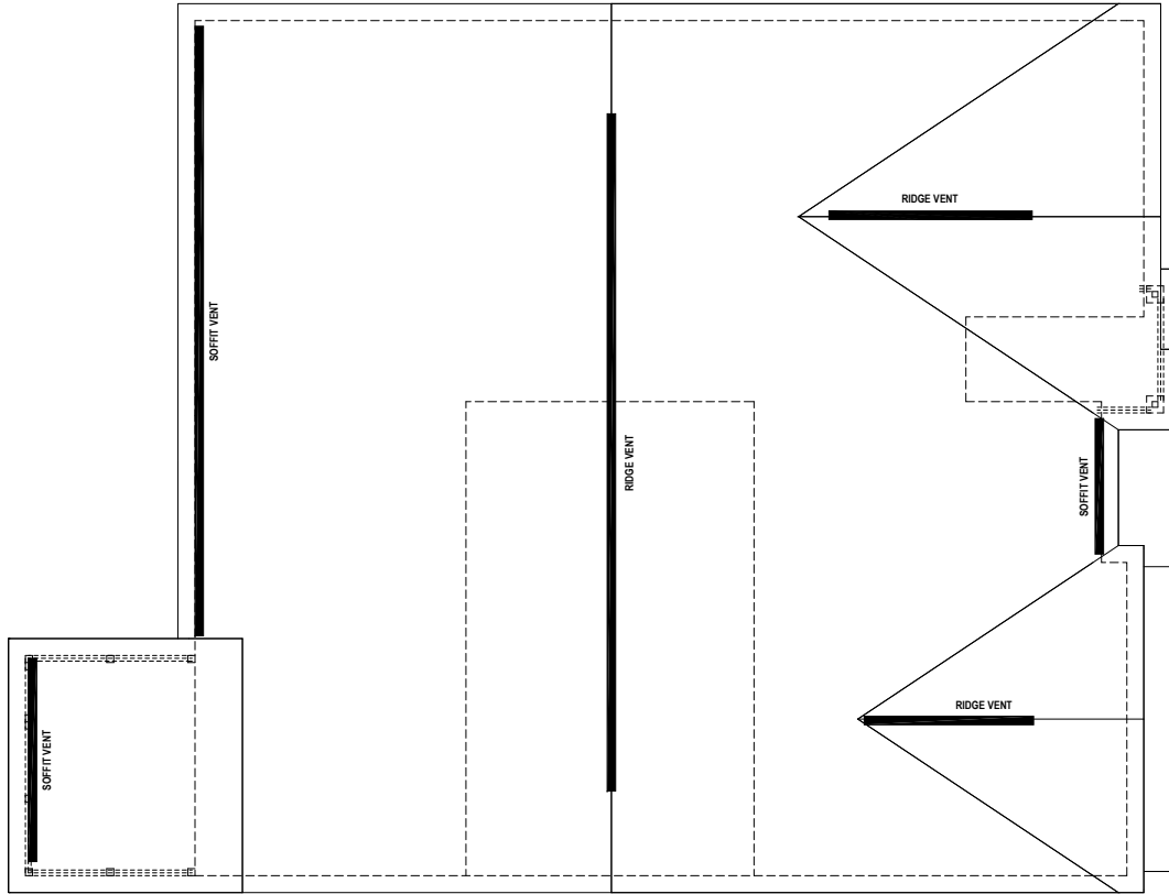
ROOF VENT PLAN "B"
