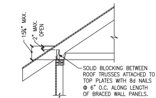
HEEL HEIGHT GREATER THAN 9 1/4" AND LESS THAN 15 1/4"
