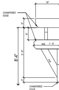
TRELLIS DETAIL
