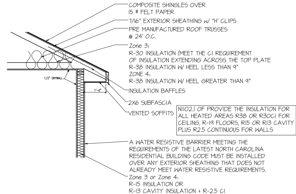
INSULATION DETAIL
