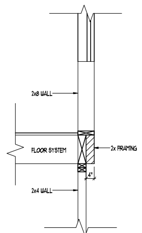
CANTILEVER DETAIL 1
