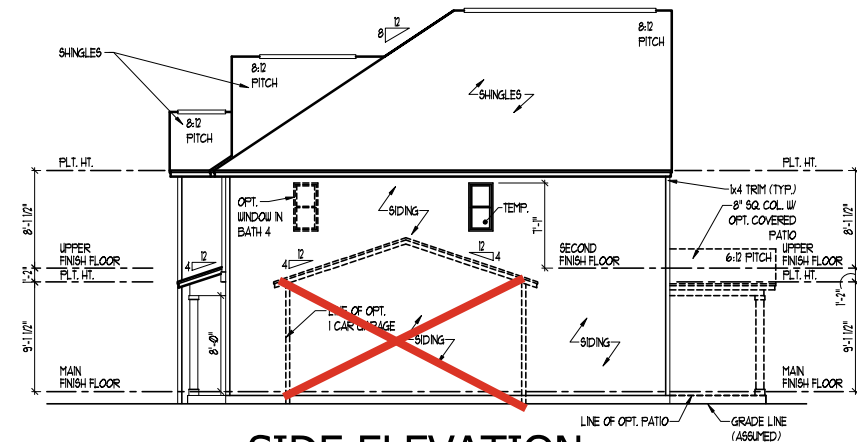
SIDE ELEVATION
