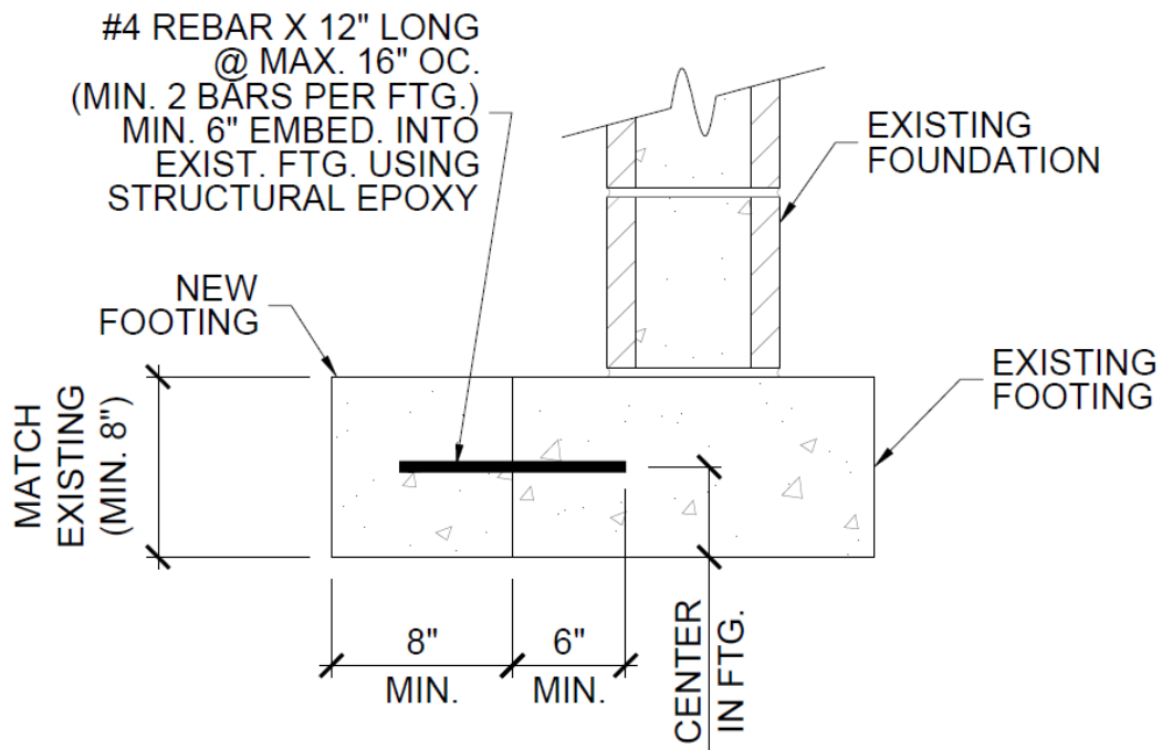
[NOT TO SCALE] EXISTING FOOTING ENLARGEMENT
