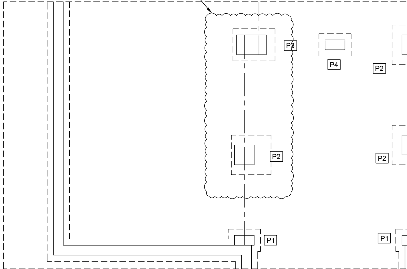
FOUNDATION PLAN SCALE: \frac{1}{4}" = 1'-0"
