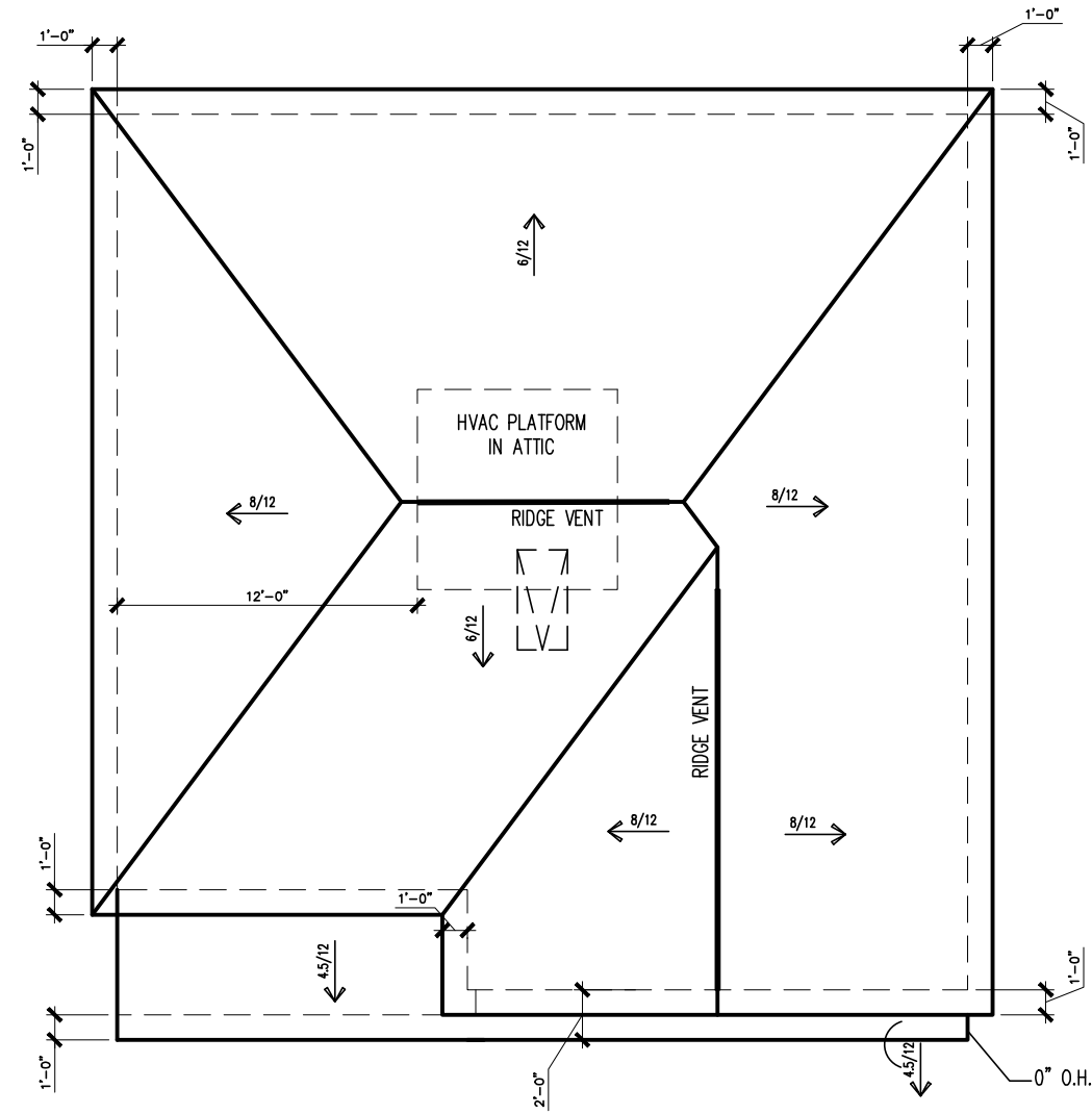
ROOF LAYOUT "C"
