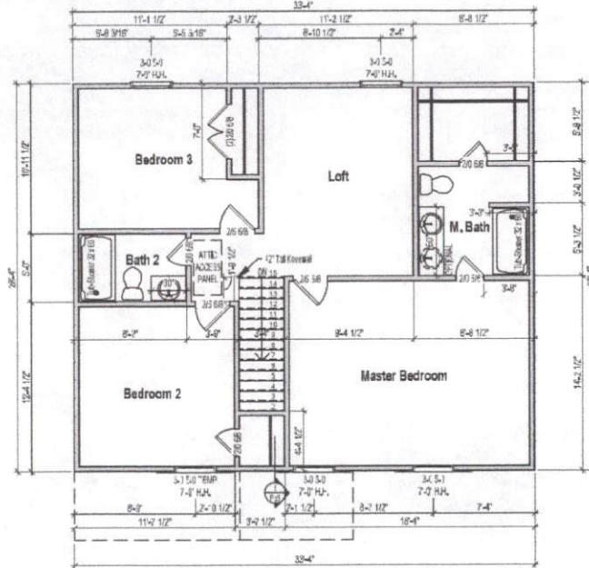
① 2nd Floor Plan - Elev A 1/8" = 1'-0"
