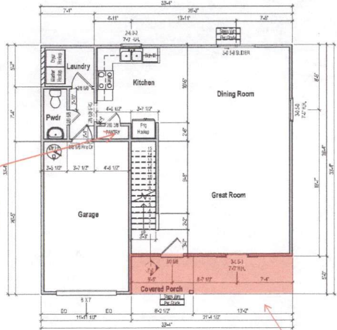
1 1st Floor Plan - Elev A 1/8" = 1'-0"
