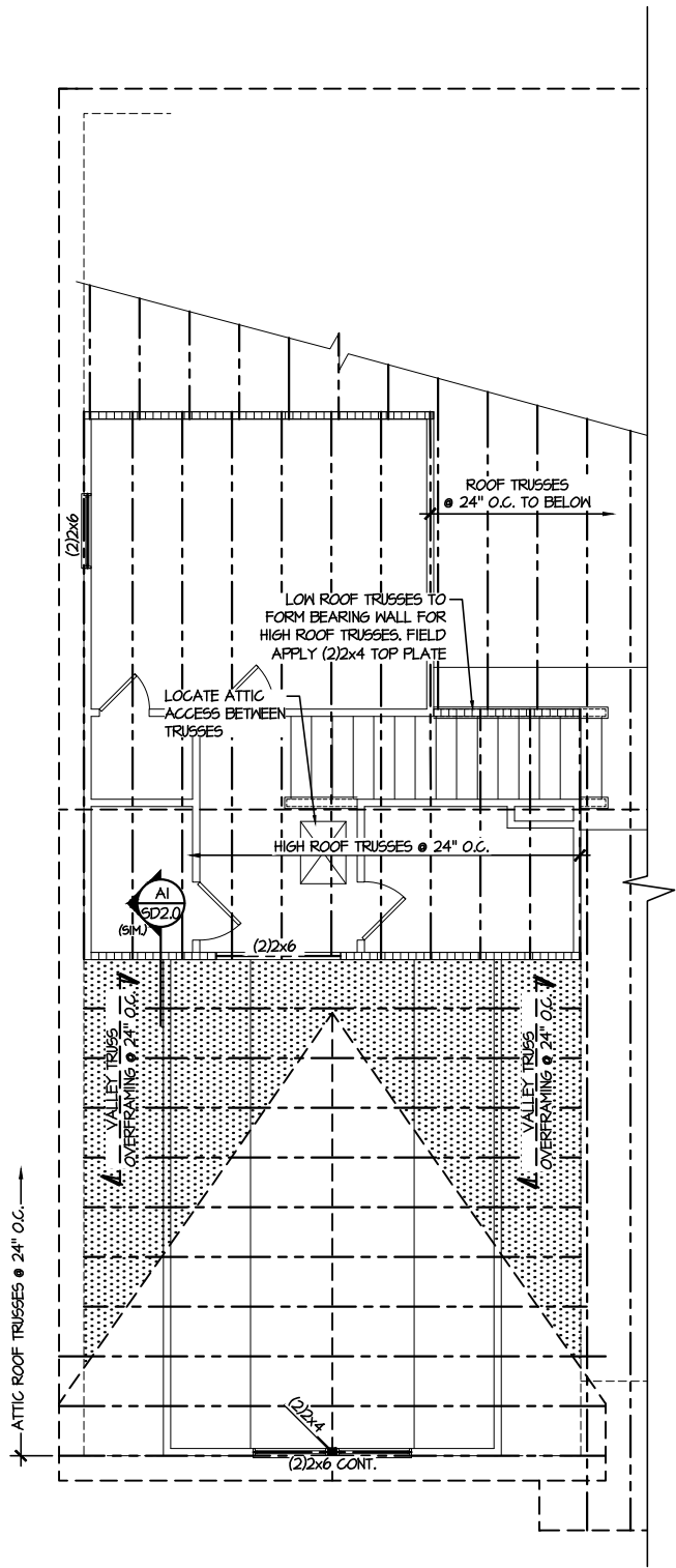
ATTIC ROOF FRAMING PLAN SCALE: 1/8"=1'-0"
