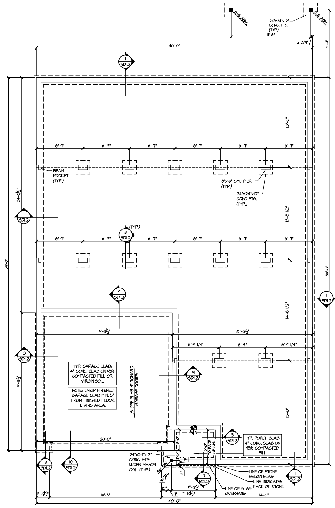
1 CRAWLSPACE FOUNDATION PLAN SCALE: 1/8"=1'-0"
