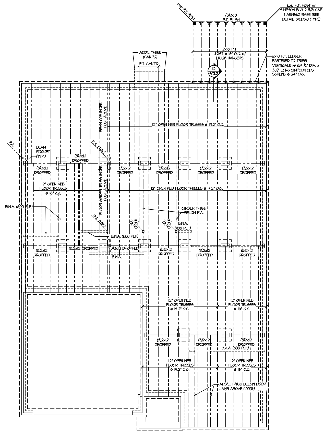
1st FLOOR FRAMING PLAN SCALE: 1/8"=1'-0"
