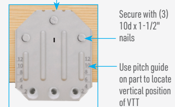
Alternate Installation for Ground / Pre-Placement installation
