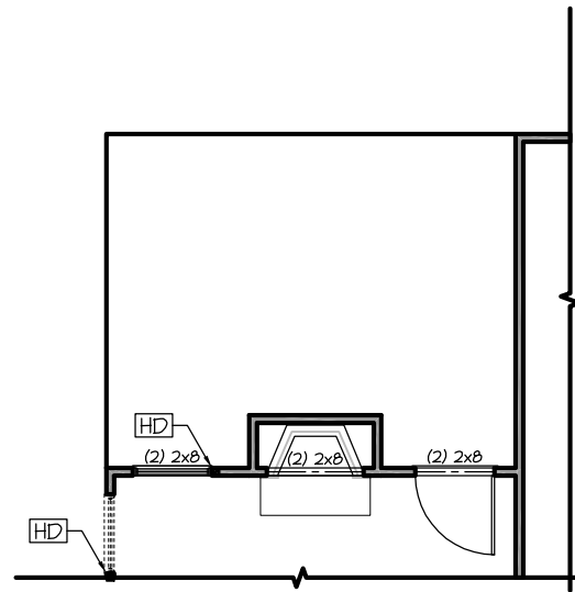
OPT. FIREPLACE
