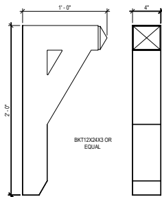
BRACKET DETAIL
