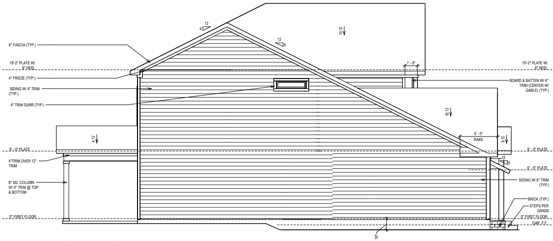
SIDE ELEVATION
