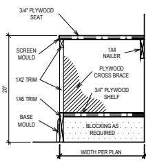
SEAT DETAIL
