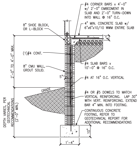
A STEM WALL TALL WALL UNBALANCED FILL 2'-0" UP TO 4'-0" MAX
