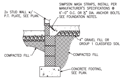
(C) FOUNDATION SECTION EXTERIOR WALL AT PORCH
