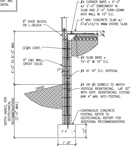
B STEM WALL TALL WALL UNBALANCED FILL 4'-0" UP TO 6'-0" MAX
