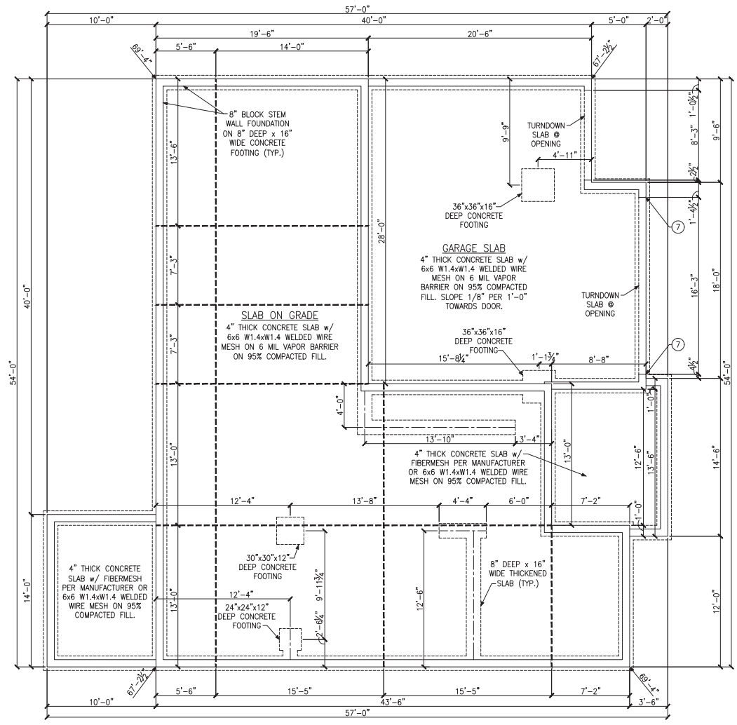
STEM WALL SLAB FOUNDATION PLAN
