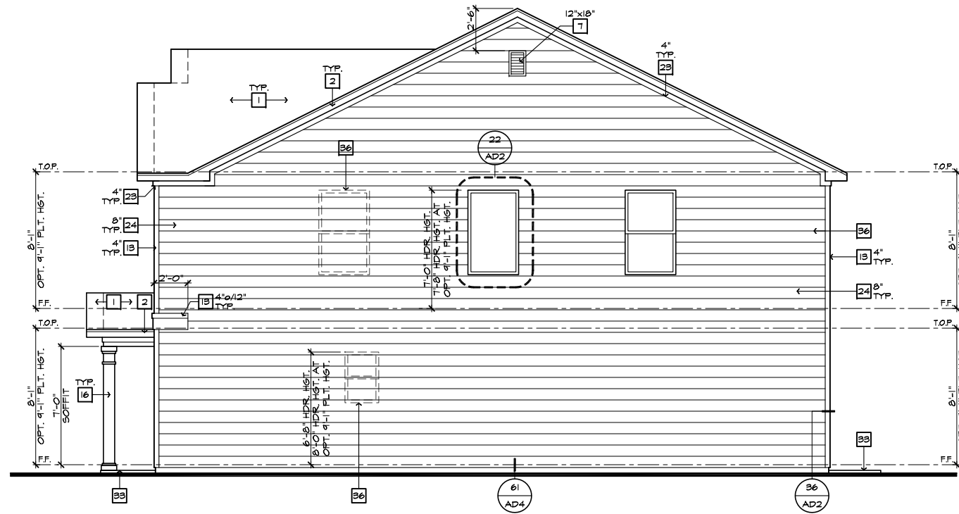
RIGHT ELEVATION 'A'
