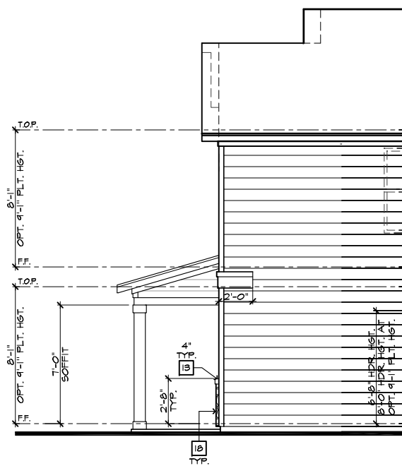
PARTIAL RIGHT ELEVATION 'C' W/ STONE OPTION
