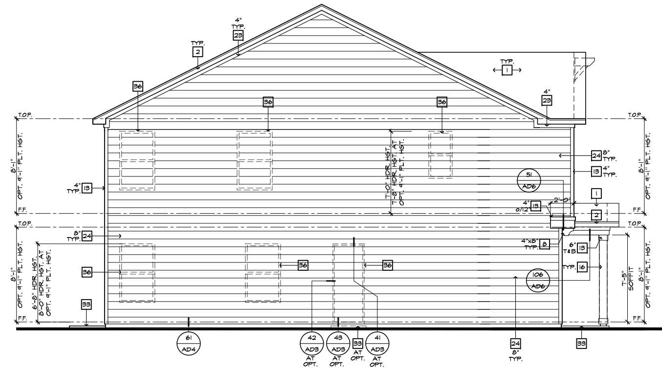
LEFT ELEVATION 'B' SCALE 1/4"=1'-0" (22'x34') - 1/8"=1'-0" (11'x17')
