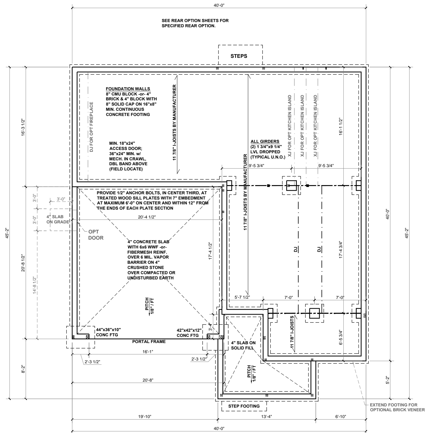
CRAWL SPACE FOUNDATION PLAN - 'C' SCALE: 1/8"=1'-0"
