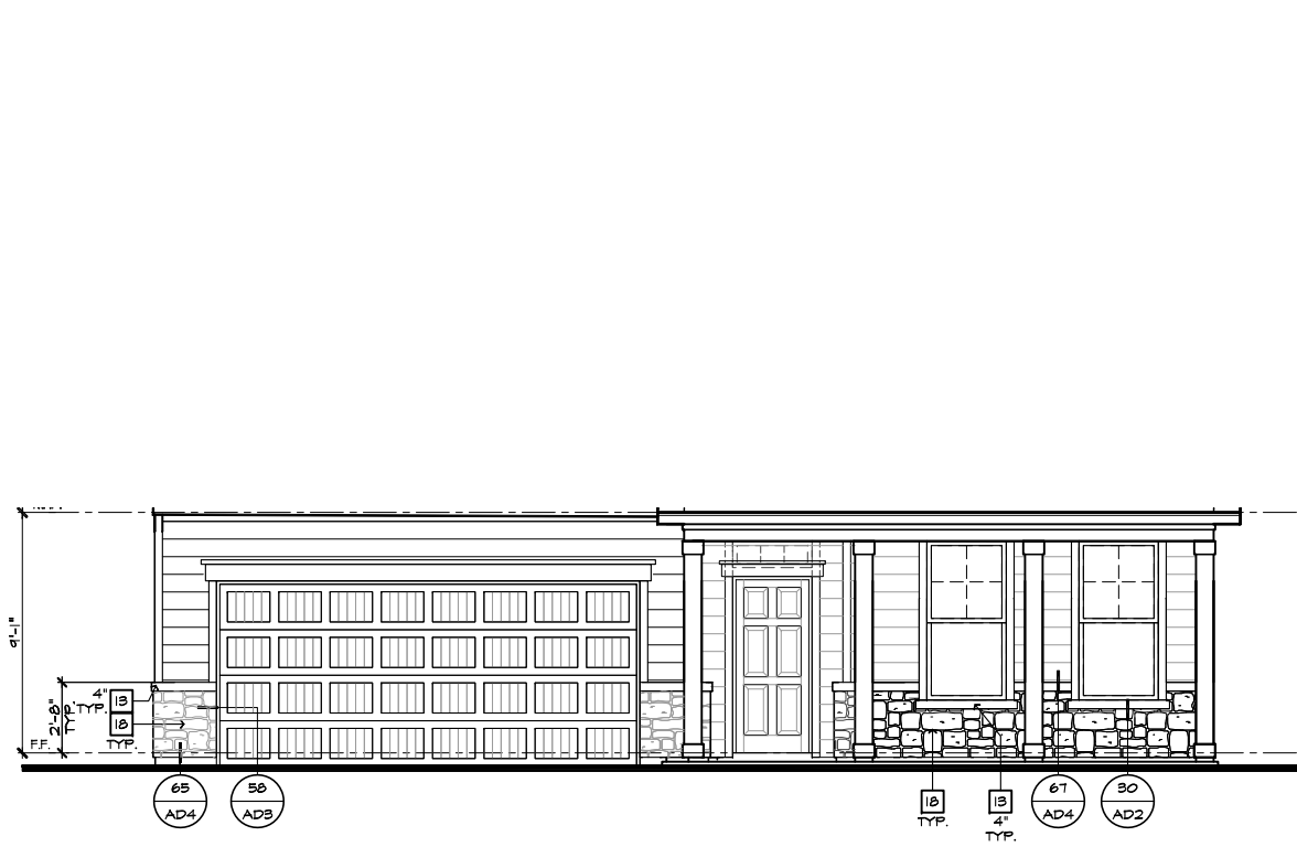
PARTIAL FRONT ELEVATION 'D' AT OPTIONAL 9'-1" PLT. HGT. W/ STONE OPT.
