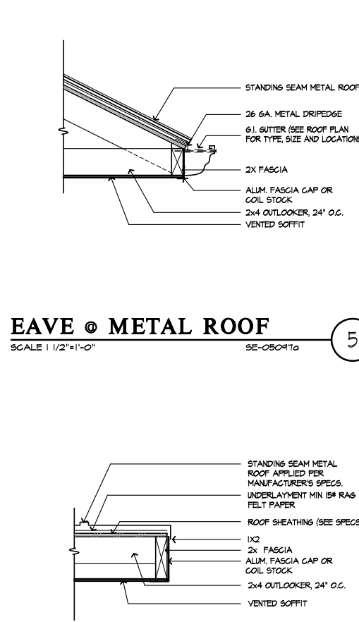
EAVE @ METAL ROOF
