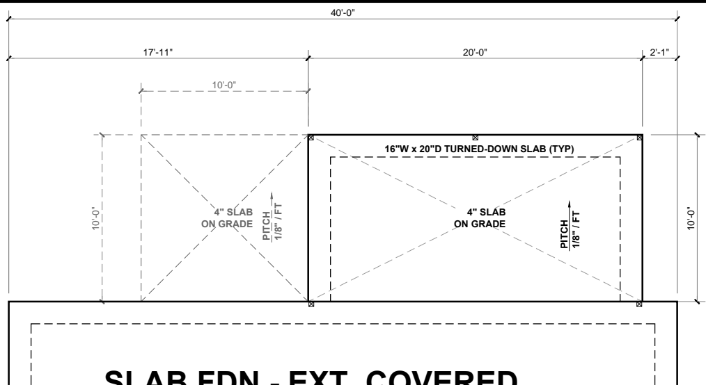
SLAB FDN - EXT. COVERED SCREENED PATIO
