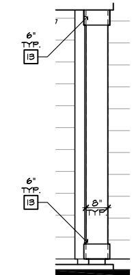
DETAIL 'D'
