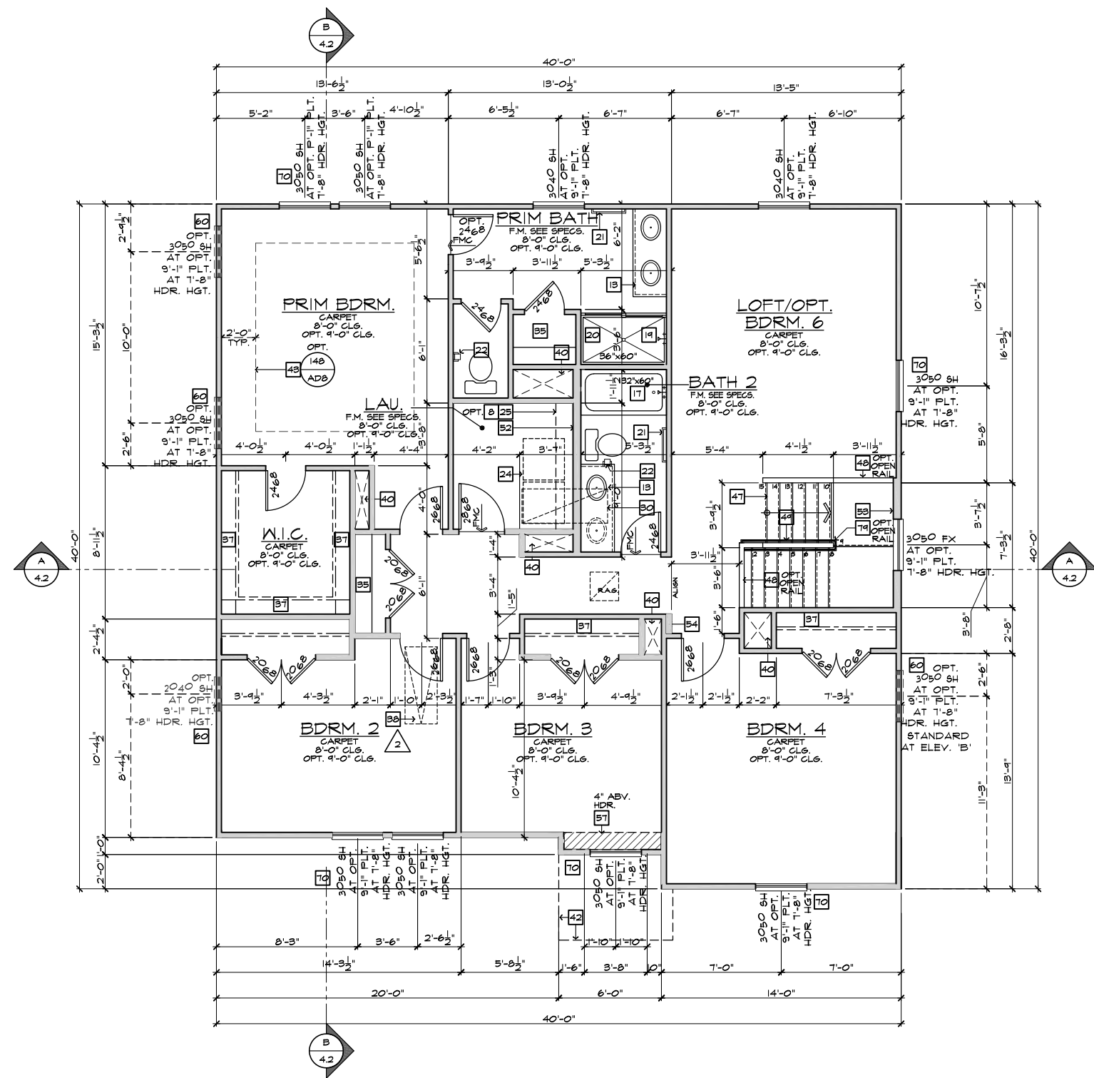
SECOND FLOOR PLAN 'A' SCALE 1/4"=1'-0" (22"X34") - 1/8"=1'-0" (16"X17") BASIC PLAN
