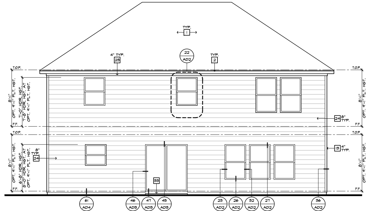
REAR ELEVATION 'D' SCALE 1/4"=1'-0" (22"X34") - 1/8"=1'-0" (11"X17")
