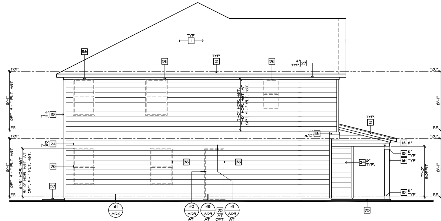
LEFT ELEVATION 'D'
