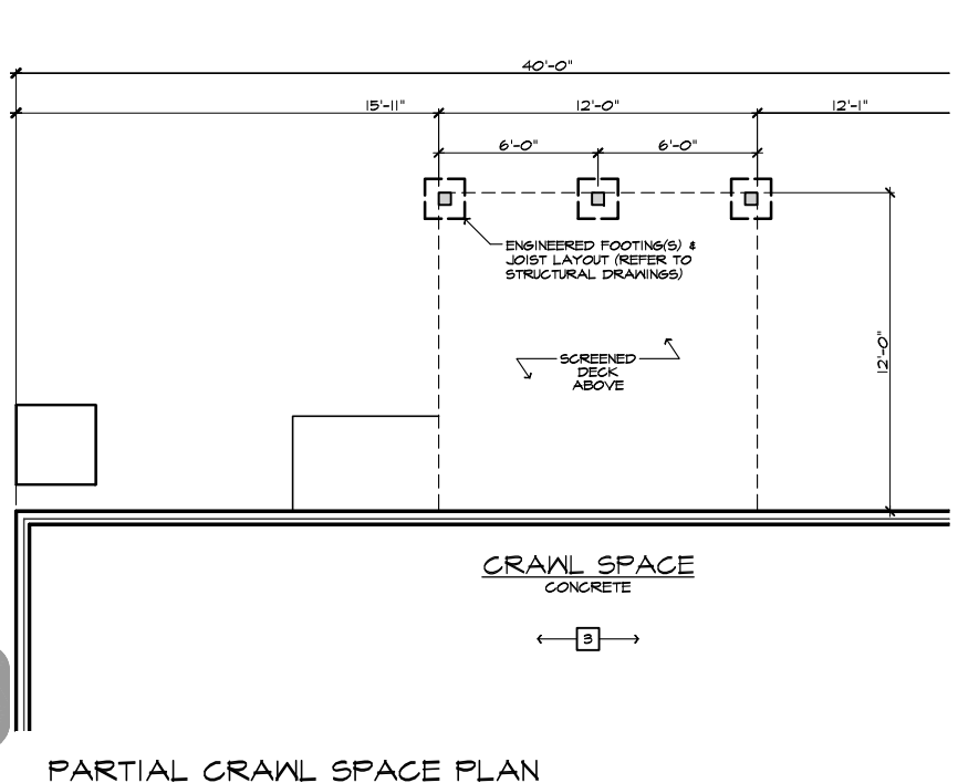
PARTIAL CRAWL SPACE PLAN
