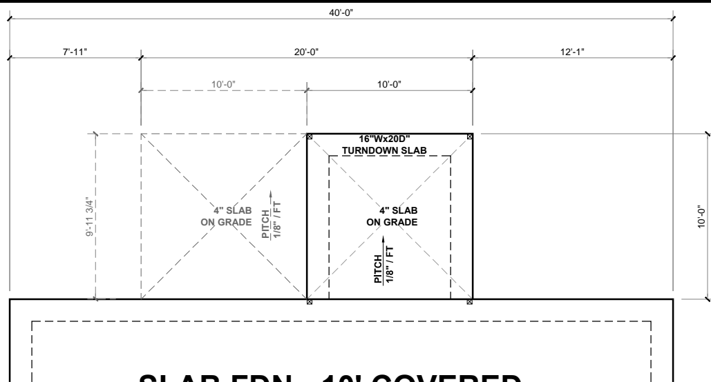
SLAB FDN - 10' COVERED SCREENED PATIO
