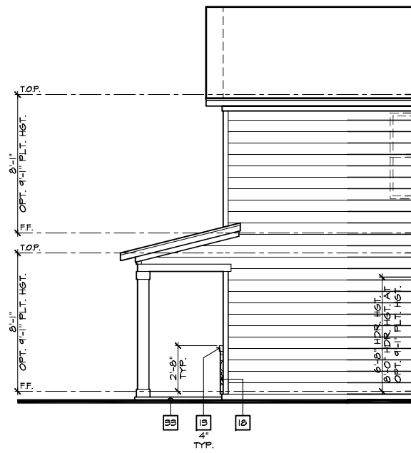
PARTIAL RIGHT ELEVATION 'D' W/ STONE OPTION
