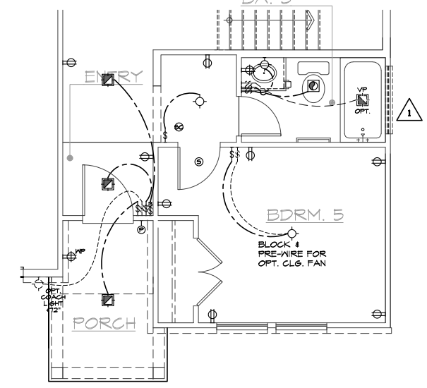
Bedroom 5 w/ Bath 3
