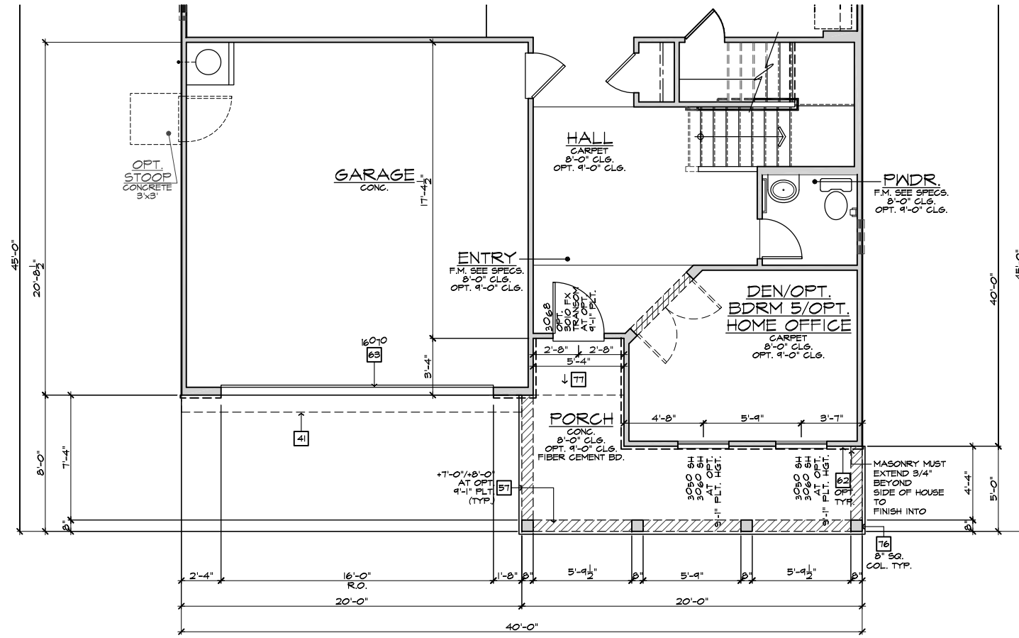
PARTIAL FIRST FLOOR PLAN 'D' SCALE 1/4"=1'-0" (22"X34") - 1/8"=1'-0" (11"X17") BASIC PLAN
