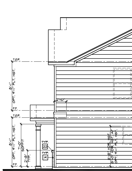
PARTIAL RIGHT ELEVATION 'A' W/ MASONRY OPTION
