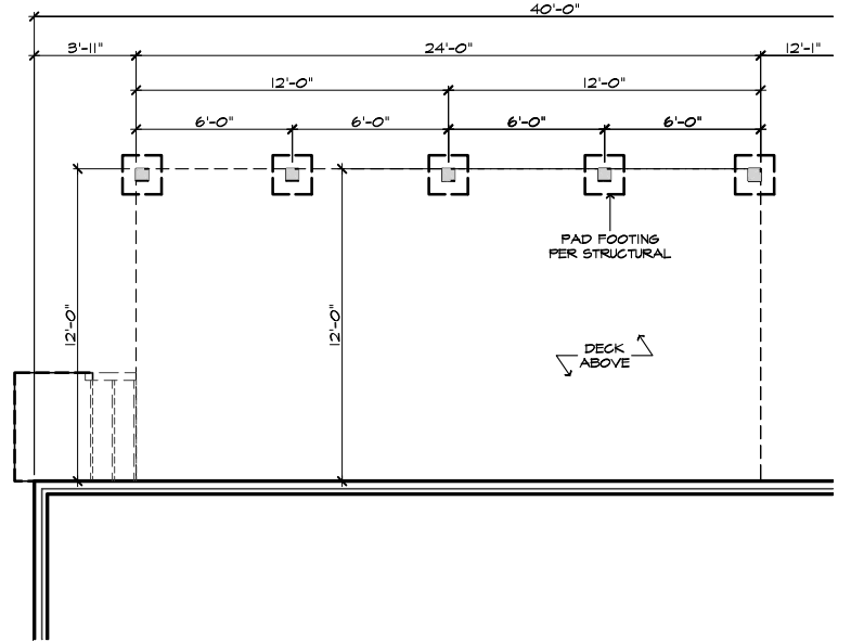
PARTIAL CRAWL SPACE PLAN
