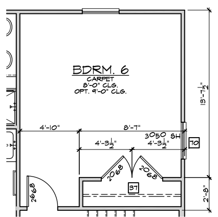
Bedroom 6 AT LOFT
