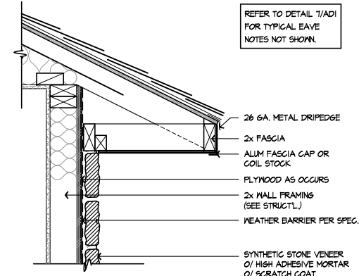
EAVE - STONE
