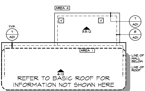
PARTIAL ROOF PLAN EXTENDED COVERED PATIO AT SLAB ON GRADE SCALE 1/4"=1'-0" (22'x34') - 1/8"=1'-0" (11'x17')
