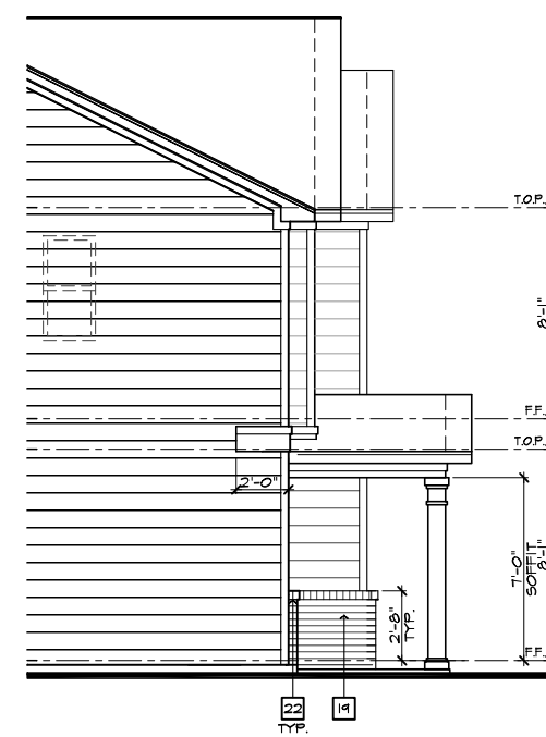
PARTIAL LEFT ELEVATION 'A' W/ MASONRY OPTION
