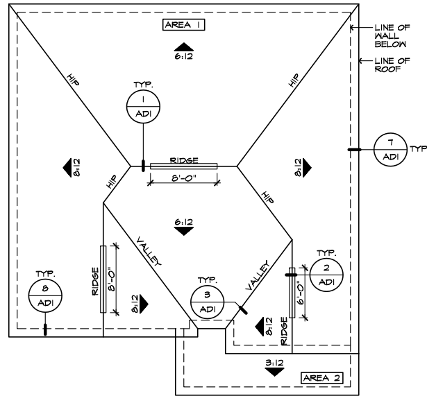
ROOF PLAN 'D' SCALE 1/8"=1'-0" (22"X34") - 1/16"=1'-0" (11"X17")
