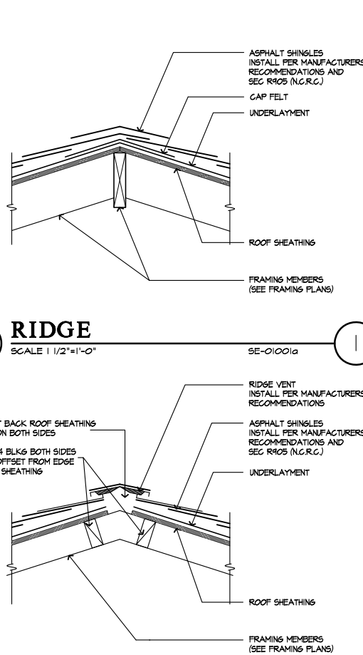
RIDGE VENT
