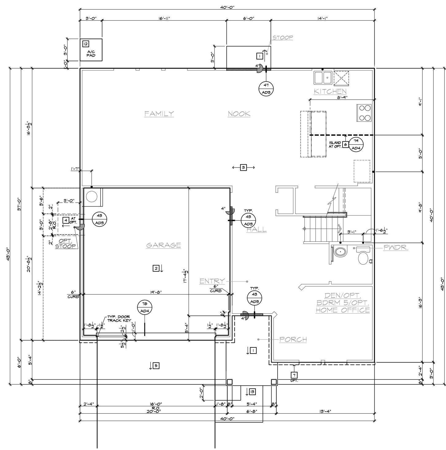
SLAB INTERFACE PLAN 'A'
