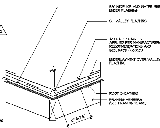
VALLEY
