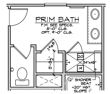
DELUXE PRIM BATH AT PRIM BATH
