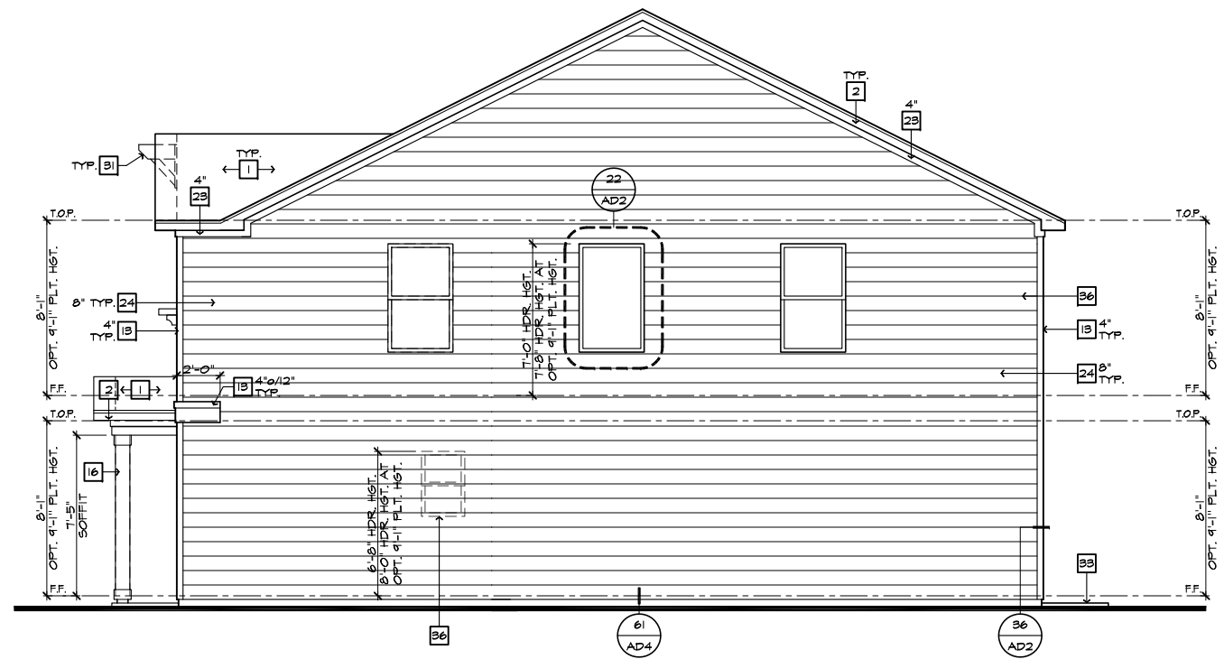
RIGHT ELEVATION 'B' SCALE 1/4"=1'-0" (22'x34') - 1/8"=1'-0" (11'x17')
