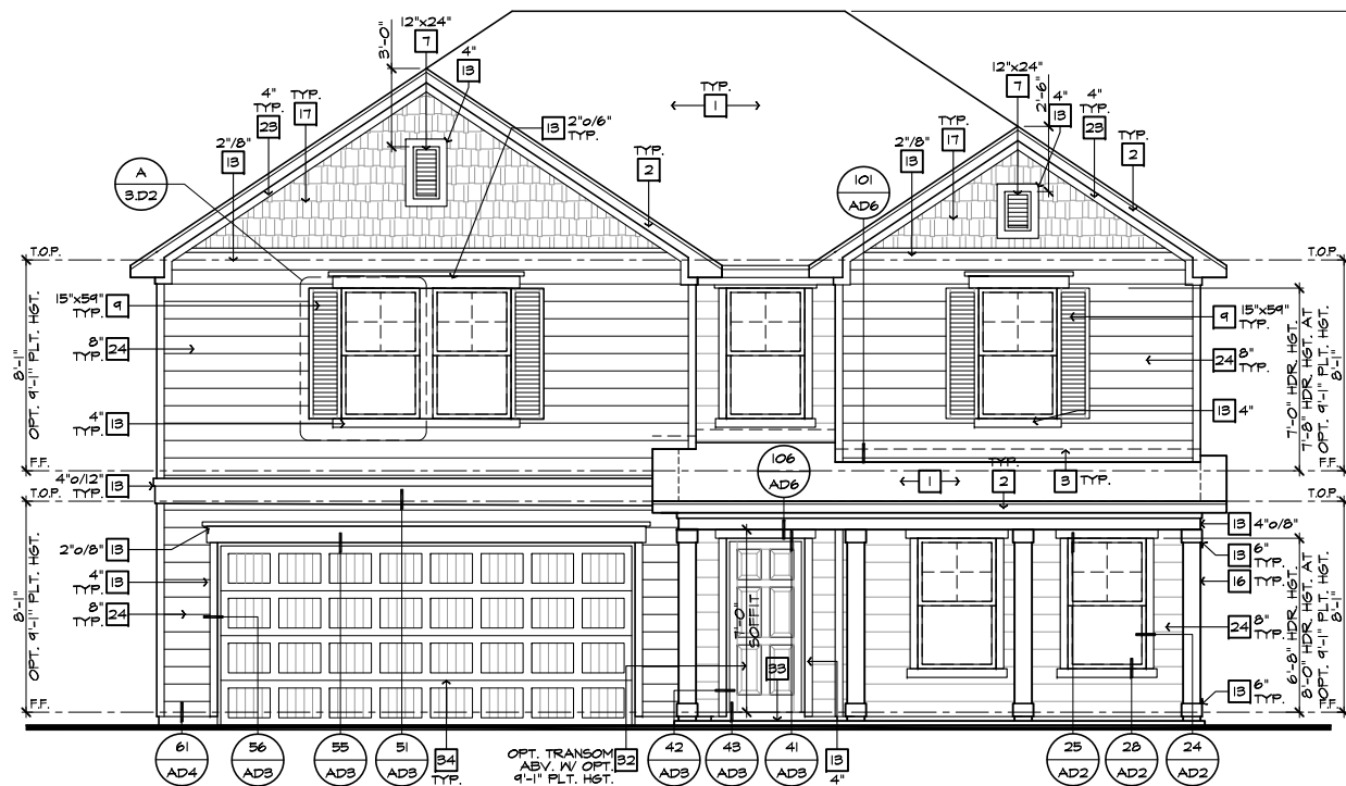
FRONT ELEVATION 'D' SCALE 1/4"=1'-0" (22"X34") - 1/8"=1'-0" (11"X17")
