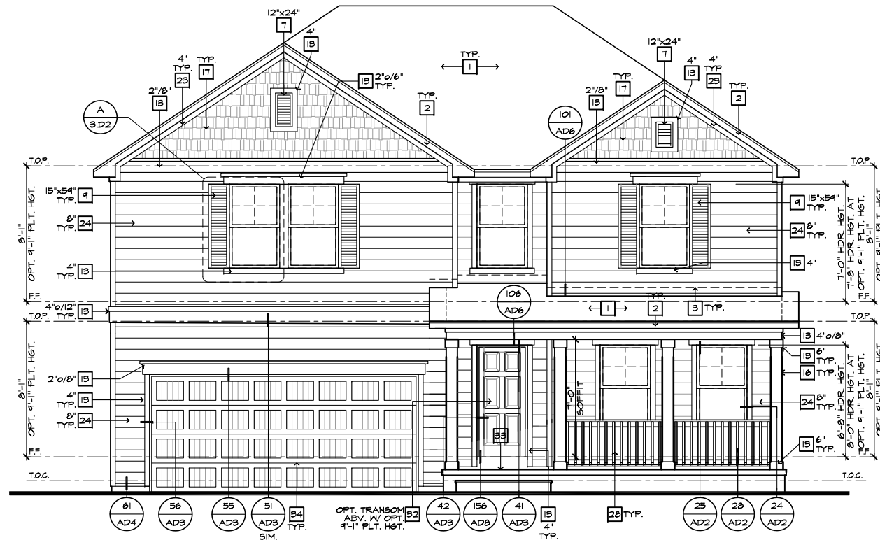
FRONT ELEVATION 'D' W/ CRAWL SPACE SCALE 1/4"=1'-0" (22'X34") - 1/8"=1'-0" (11'X17')
