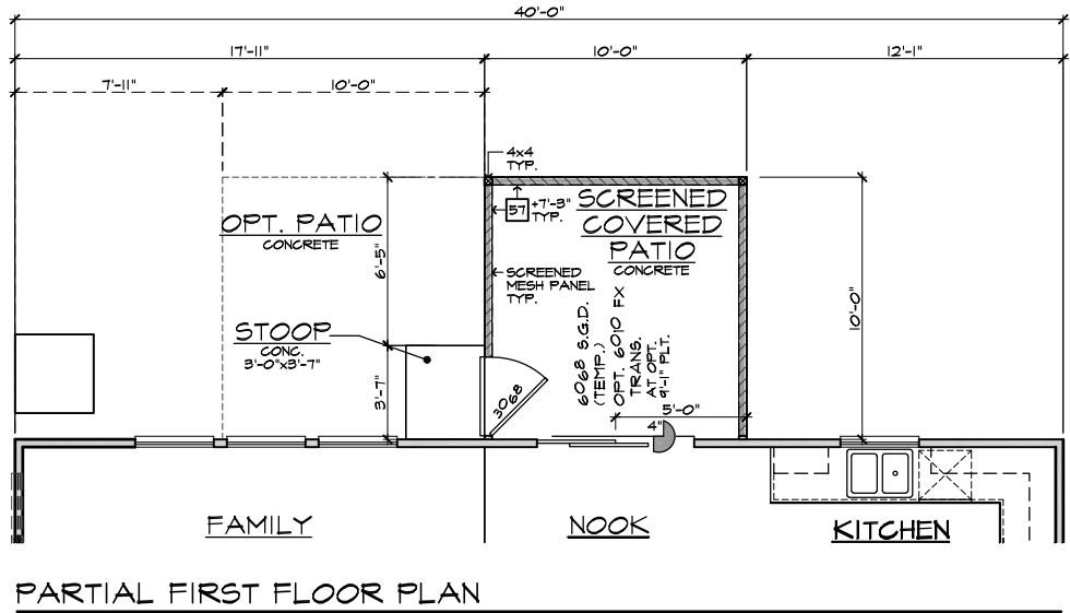
PARTIAL SLAB INTERFACE PLAN
