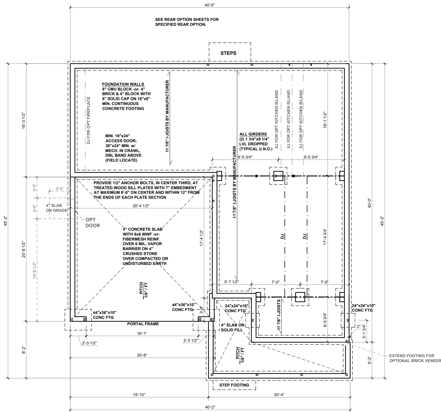
CRAWL SPACE FOUNDATION PLAN - 'D' SCALE: 1/8"=1'-0"
