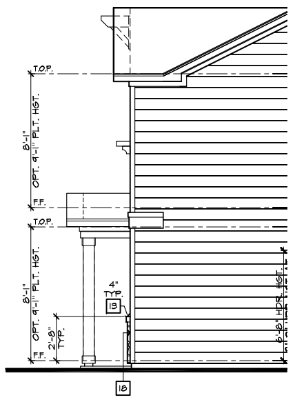
PARTIAL RIGHT ELEVATION 'B' W/ STONE OPTION SCALE 1/4"=1'-0" (22'x34') - 1/8"=1'-0" (11'x17')
