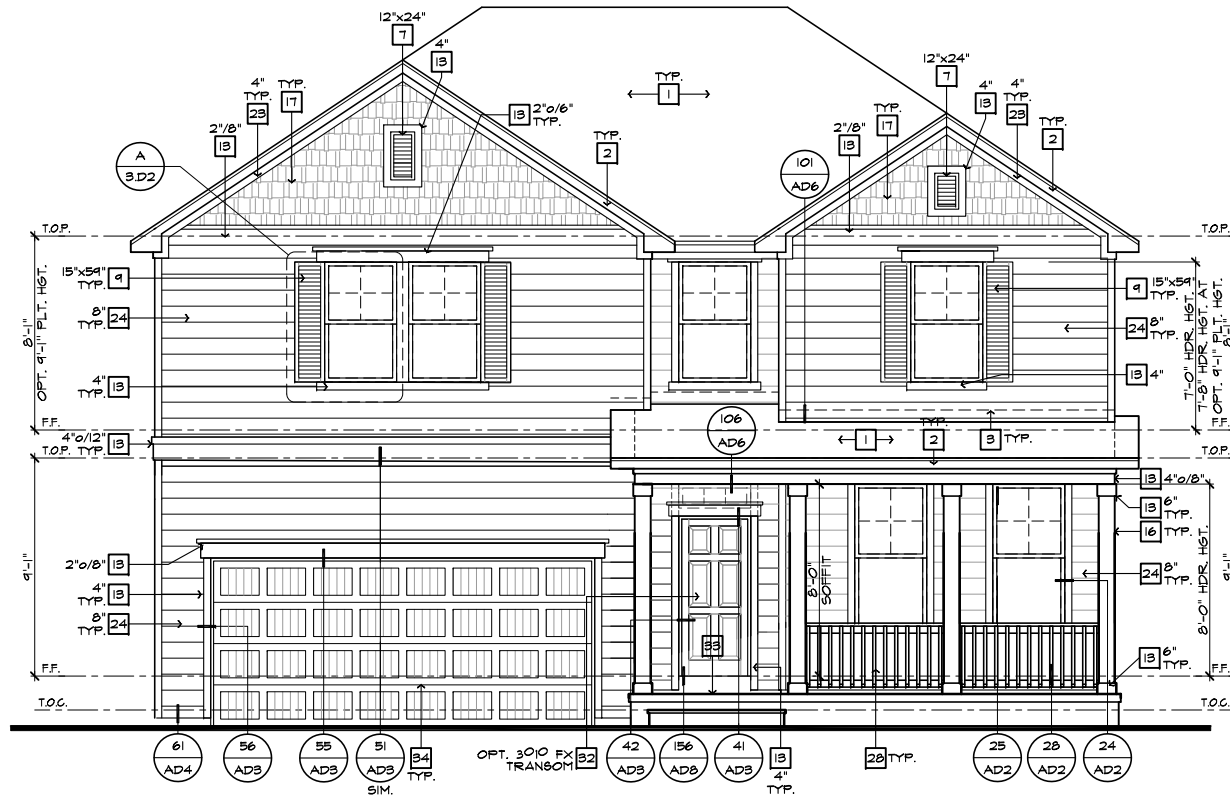
FRONT ELEVATION 'D' W/ CRAWL SPACE AT OPTIONAL 9'-1" PLT. HGT.
