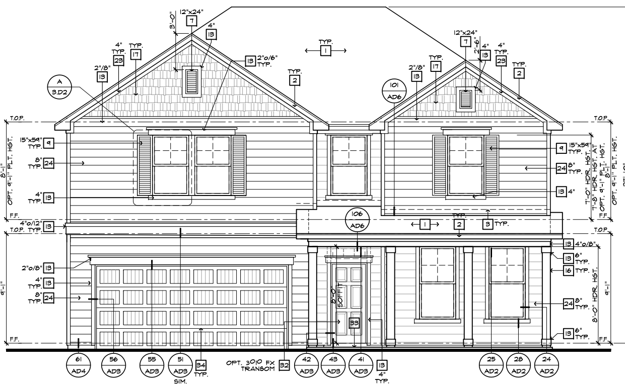
FRONT ELEVATION 'D' AT OPTIONAL 9'-1" PLT. HGT.
