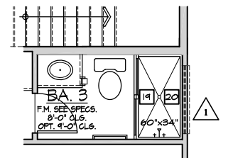
SHOWER I.L.O. TUB AT BATH 3
