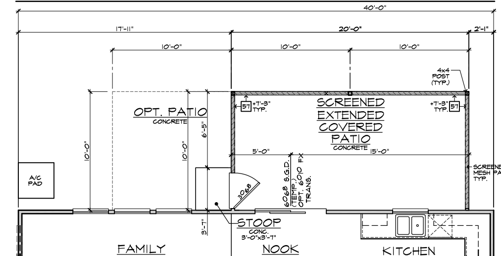
PARTIAL FIRST FLOOR PLAN
