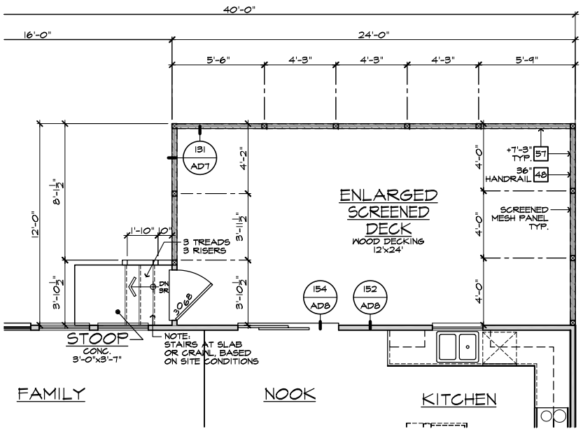
PARTIAL FIRST FLOOR PLAN
