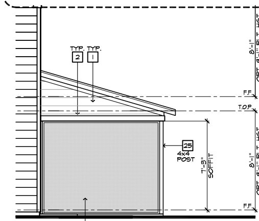
PARTIAL RIGHT ELEVATION
