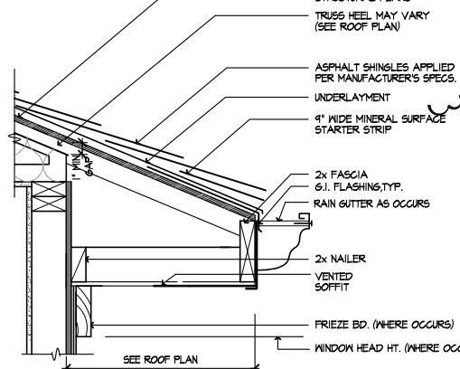
EAVE
