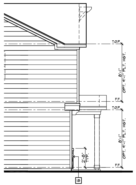
PARTIAL LEFT ELEVATION 'B' W/ STONE OPTION SCALE 1/4"=1'-0" (22'x34') - 1/8"=1'-0" (11'x17')
