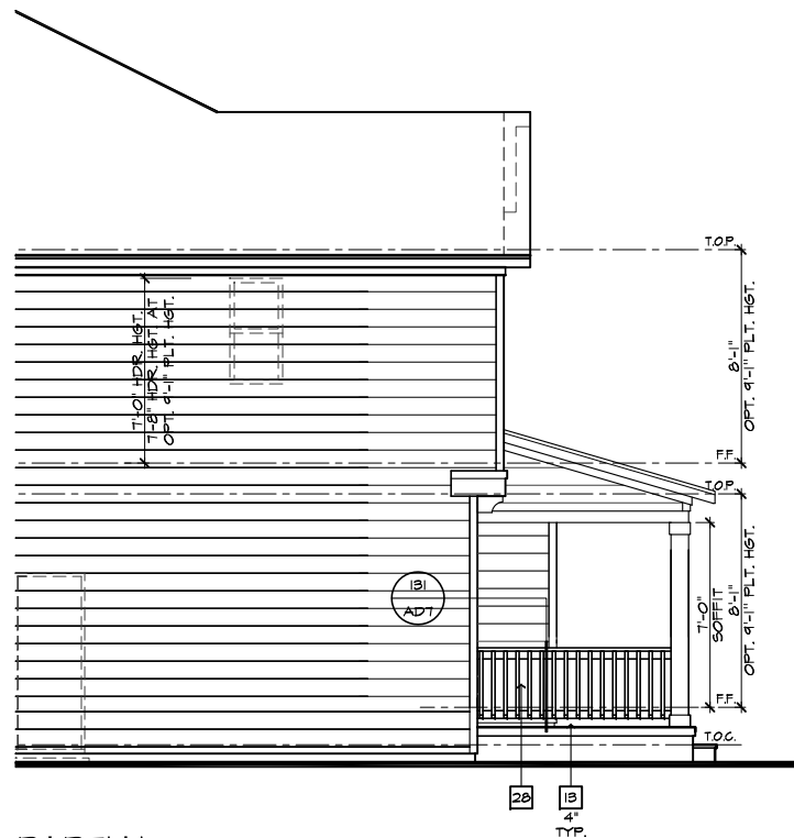
PARTIAL LEFT ELEVATION 'C' AT CRAWL SPACE SCALE 1/4"=1'-0" (22'x34') - 1/8"=1'-0" (11'x17')
