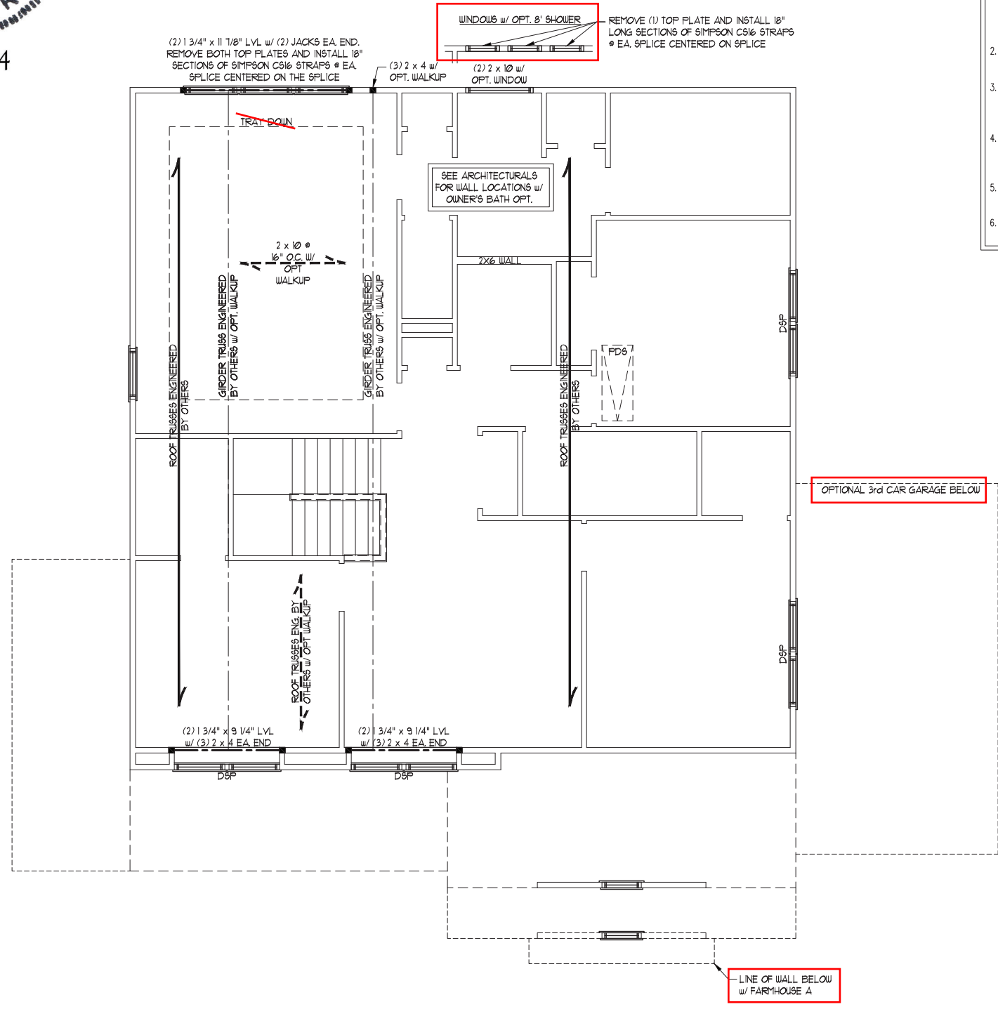
BUNGALOW A / FARMHOUSE A
