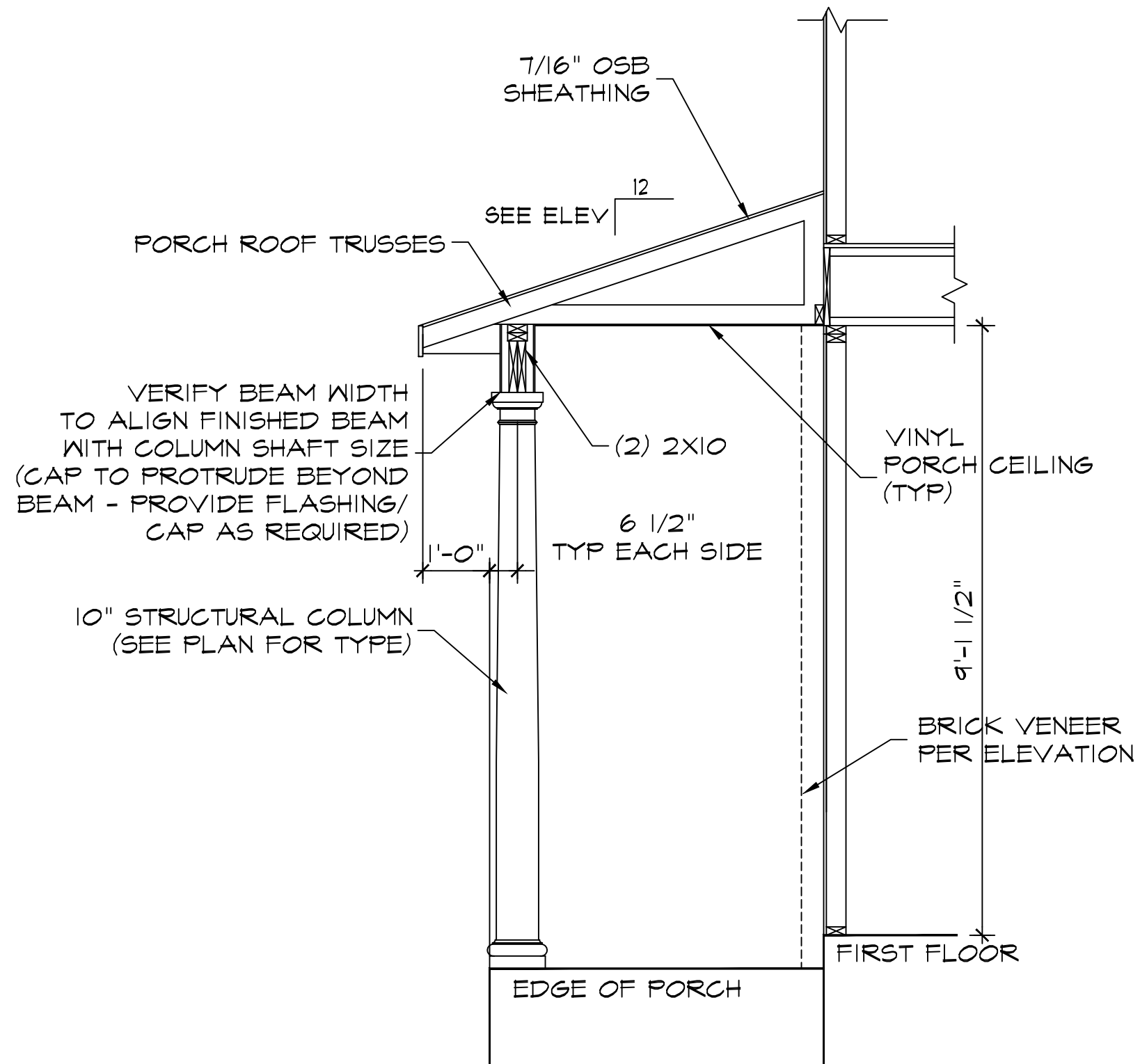
PORCH DETAIL 1/2" = 1'-0" FARMHOUSE
