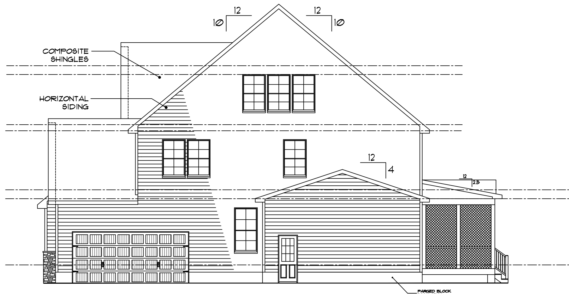
RIGHT ELEVATION - FARMHOUSE A
