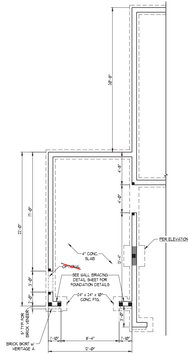
OPT 3 CAR GARAGE w/ FRONT LOAD 2-CAR GARAGE
