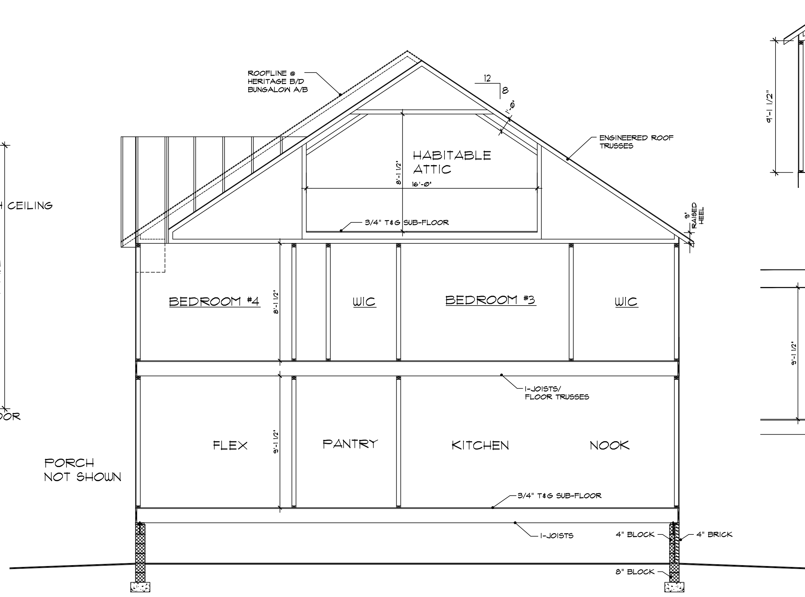
1 A-7 TYPICAL HOUSE SECTION 1/4" = 1'-0" CRAWL SPACE
