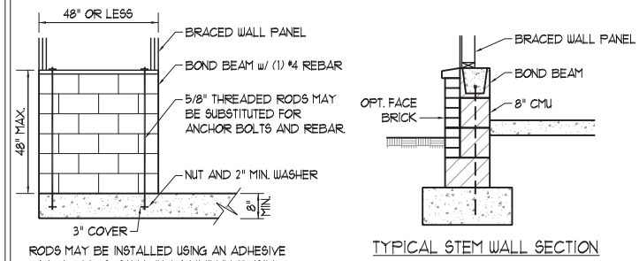
NOTE: GROUT BOND BEAMS AND ALL CELLS WHICH CONTAIN REBAR, THREADED RODS AND ANCHOR BOLTS MASONRY STEM WALLS SUPPORTING BRACED WALL PANELS (2) PER FIGURE R602.10.4.3
