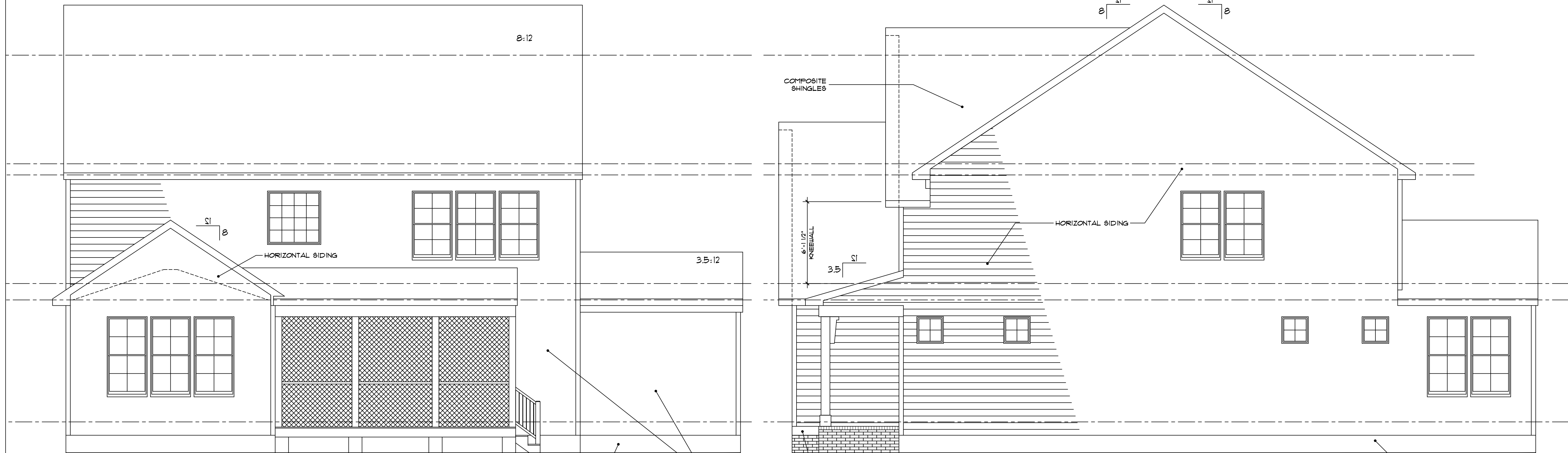
REAR ELEVATION - FARMHOUSE A
