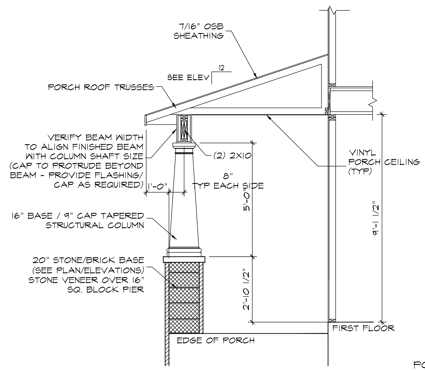
2 A-8 PORCH DETAIL 1/2" = 1'-0" BUNGALOW
