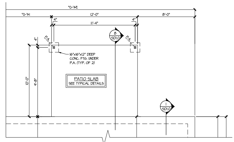
2 PARTIAL MONO-SLAB FOUNDATION PLAN SCALE: 1/4"=1'-0" ON 22x34 1/8"=1'-0" ON 11x17 OPT. COVERED PATIO ALL ELEVS. SIM. SEE BASE ELEV. FOR ADD'L INFO.
