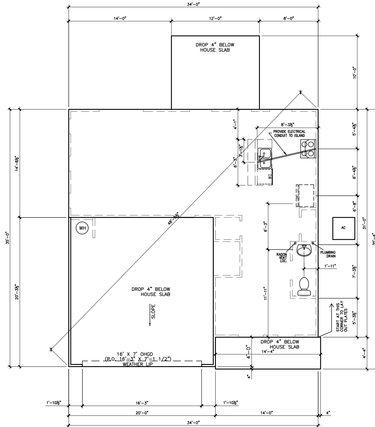
SLAB PLAN
