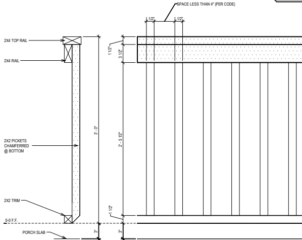
RAIL DETAIL 'A' SCALE: 1" = 1'-0"
