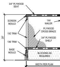
SEAT DETAIL
