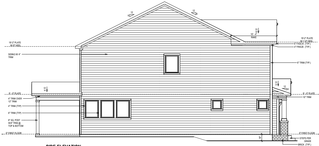
SIDE ELEVATION
