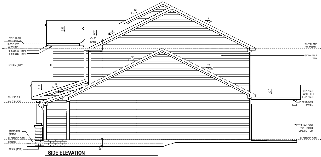
SIDE ELEVATION
