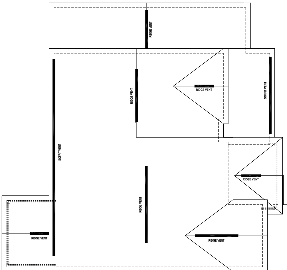
ROOF PLAN W/COVERED PORCH CALCS
