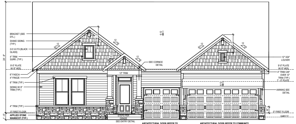
FRONT ELEVATION
