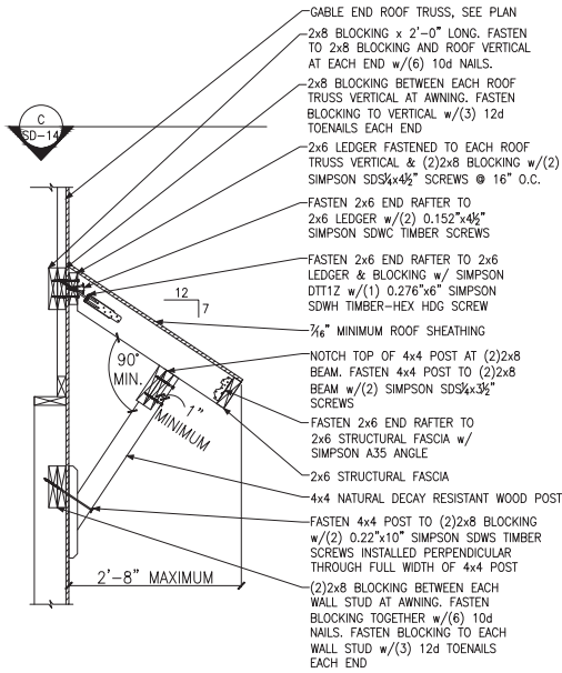
A PORCH AWNING SECTION END RAFTER
