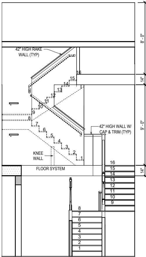
STAIR SECTION
