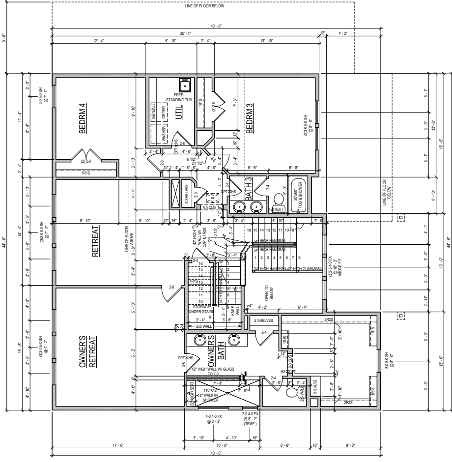
SECOND FLOOR
