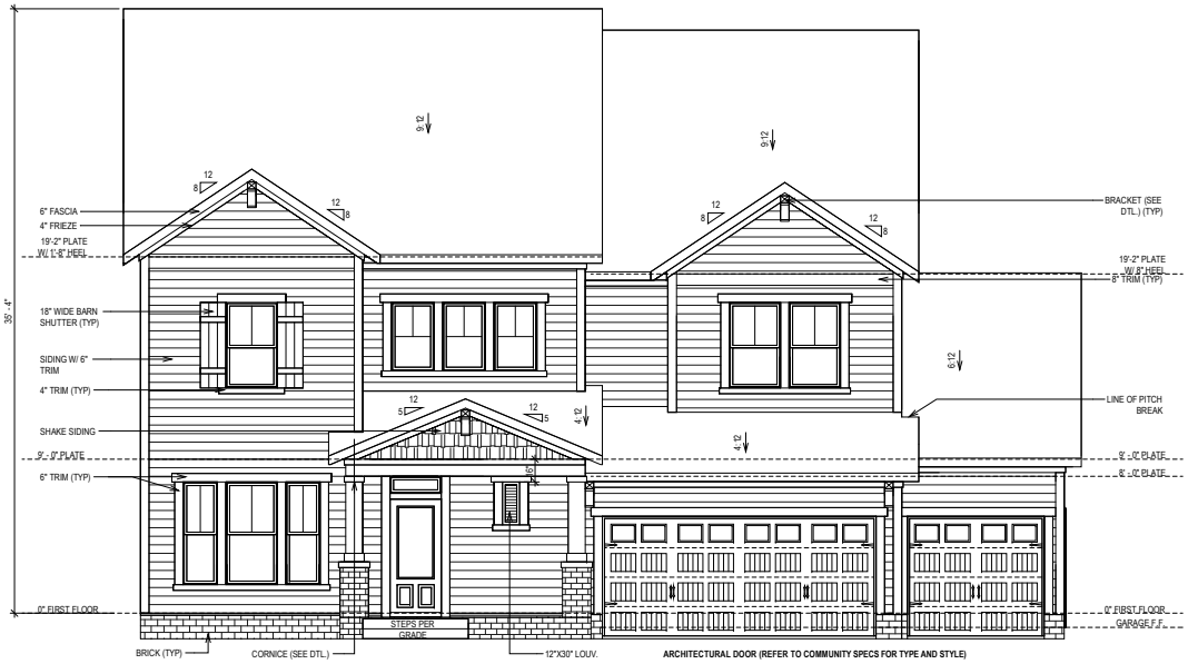
FRONT ELEVATION "B" CRAFTSMAN
