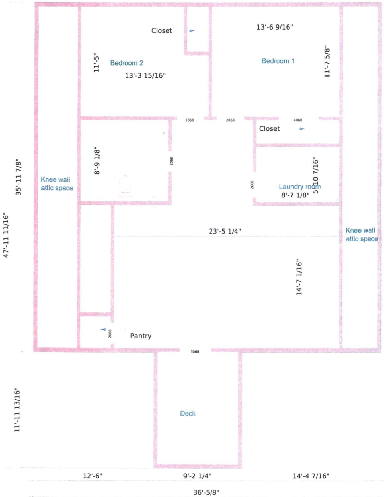
Second Level floor plan
