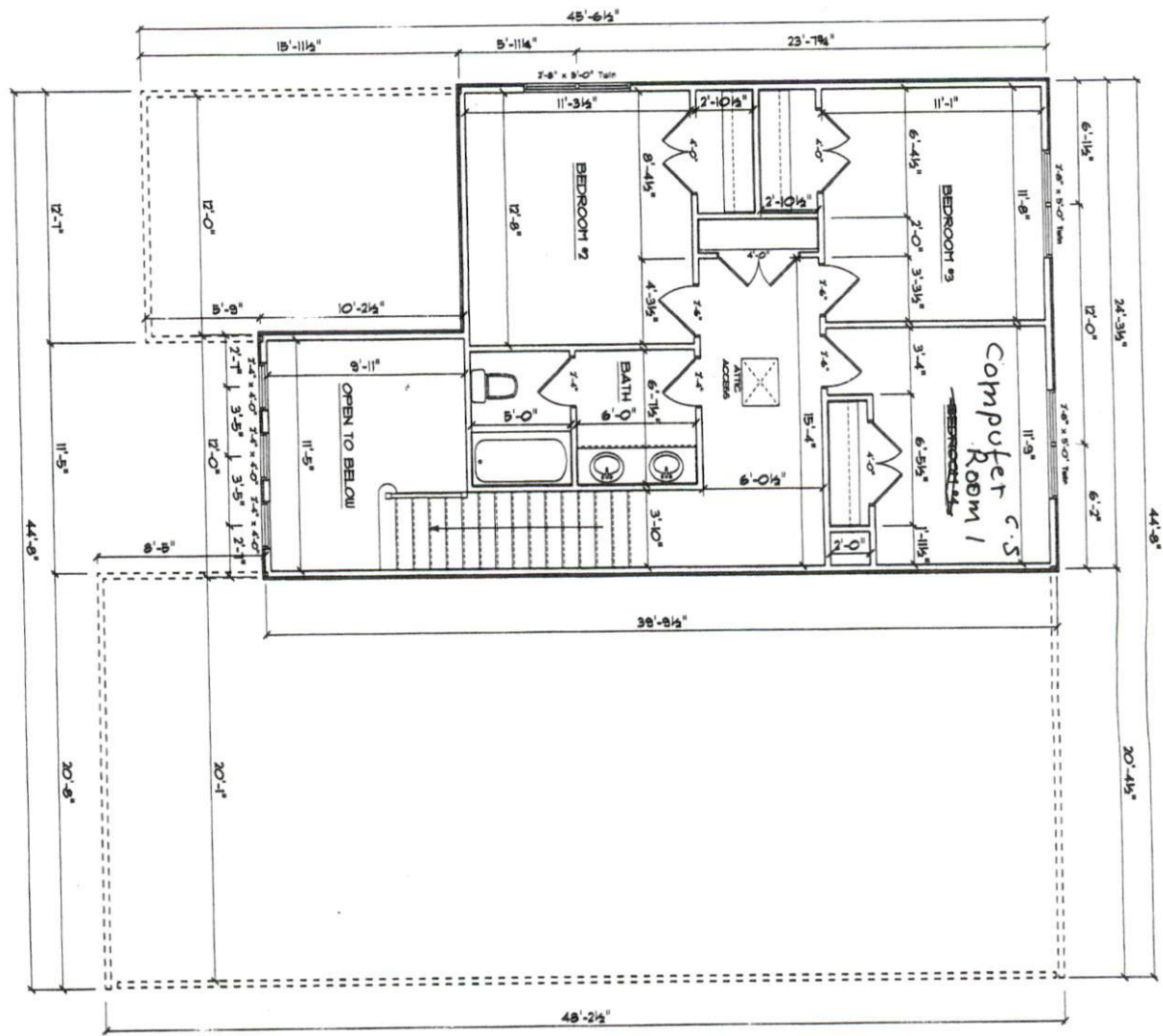
2ND FLOOR PLAN SCALE: 1" = 1/4"
