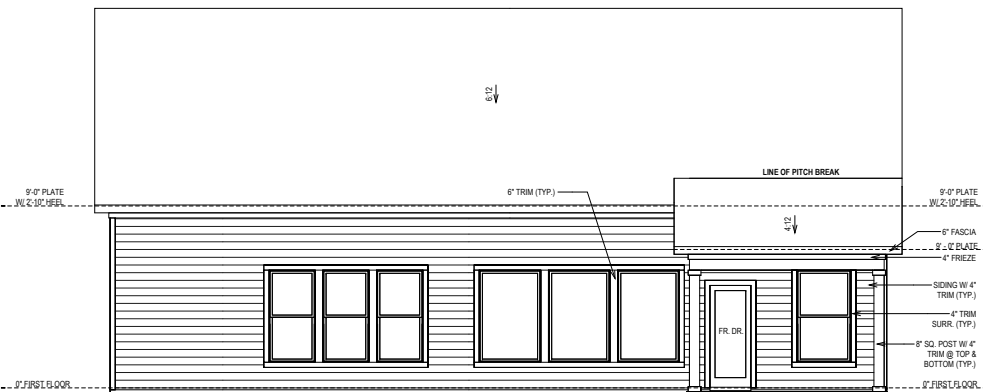
REAR ELEVATION
