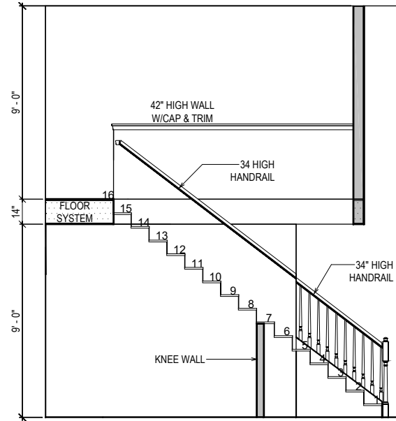
STAIR SECTION
