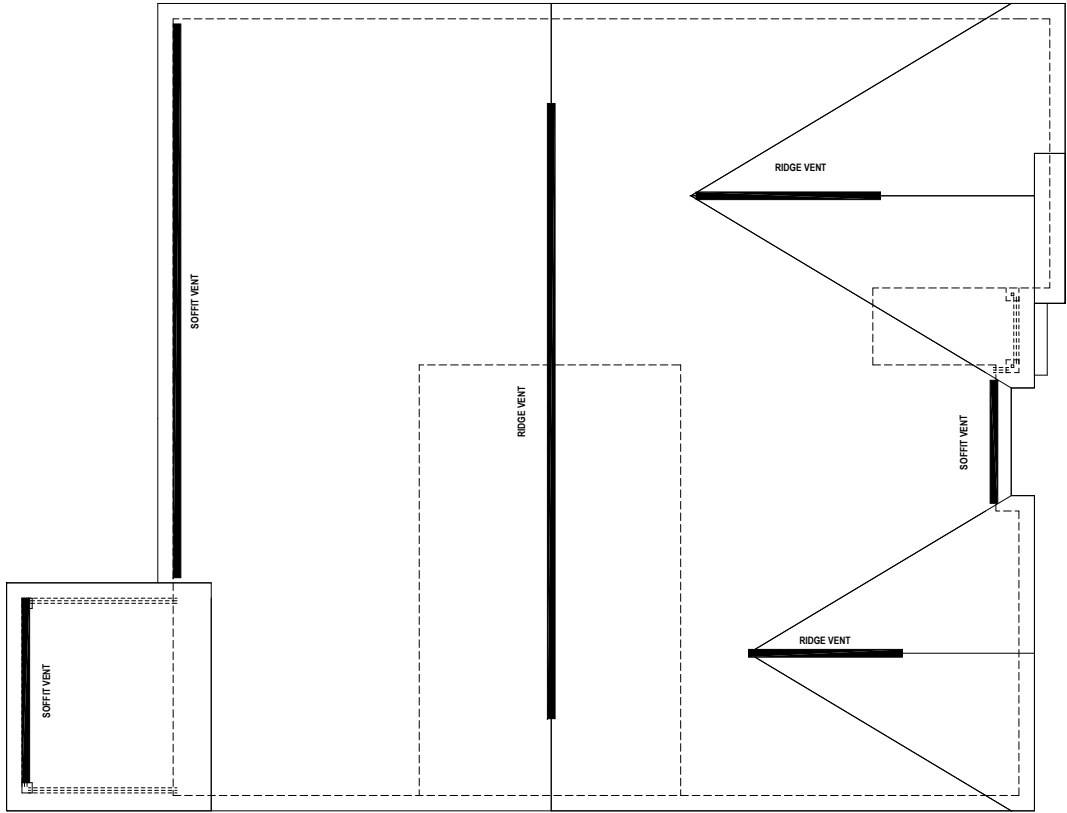
ROOF PLAN VENT CALCS "A"
