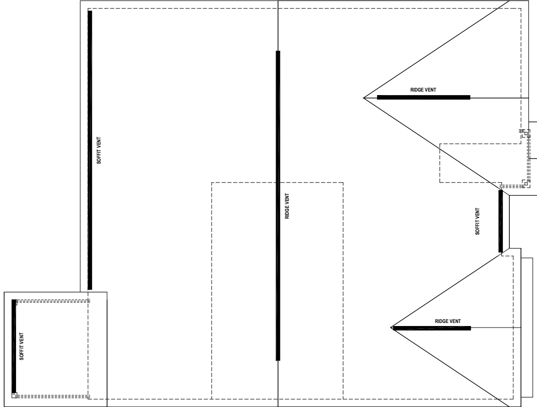
ROOF PLAN CALCS "B"
