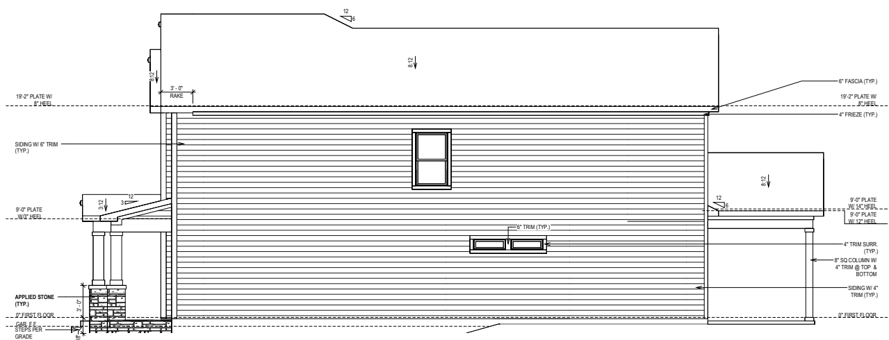
SIDE ELEVATION
