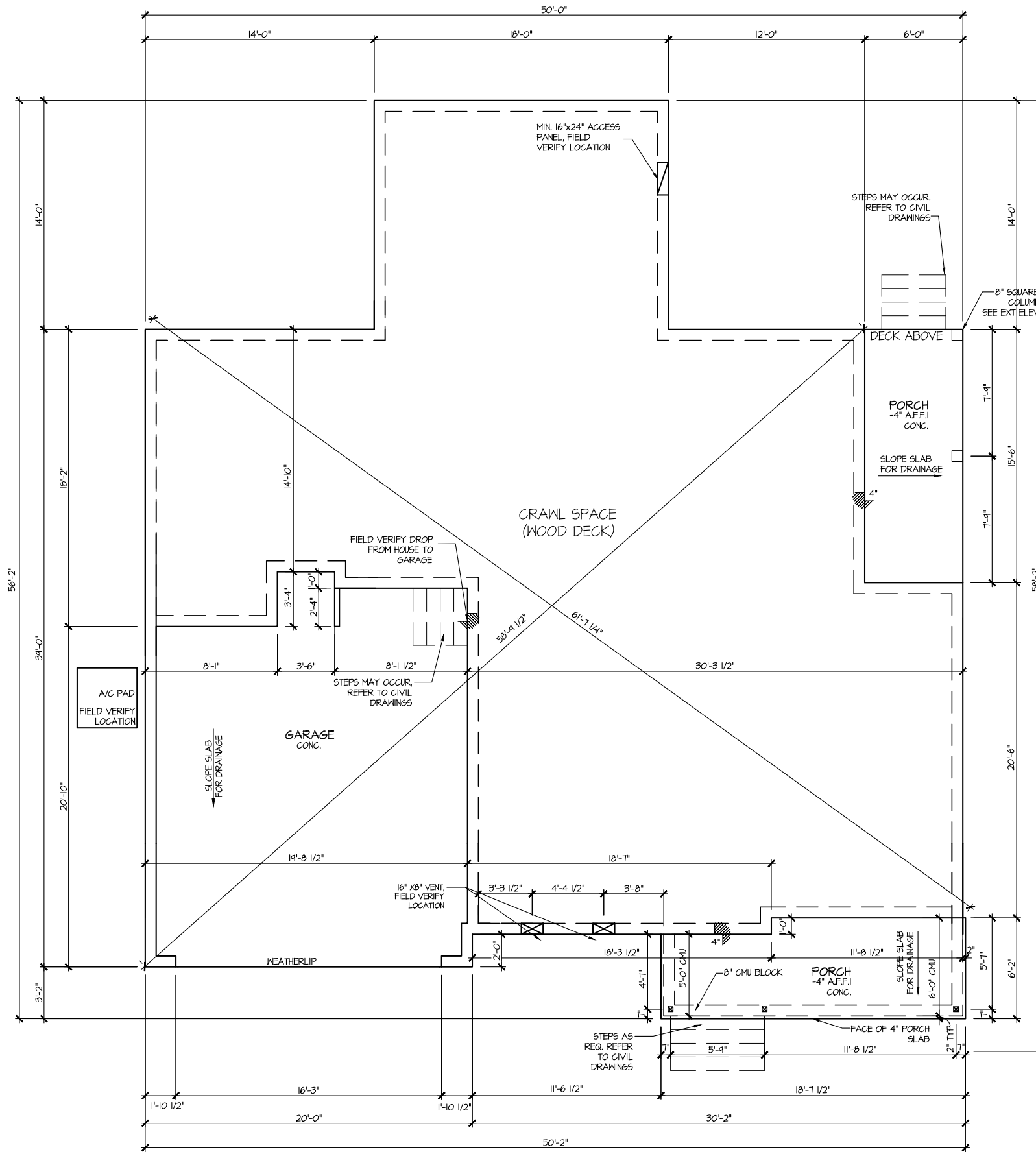
ELEVATION 1 CRAWL SPACE PLAN SCALE: 1/8" = 1'-0"
