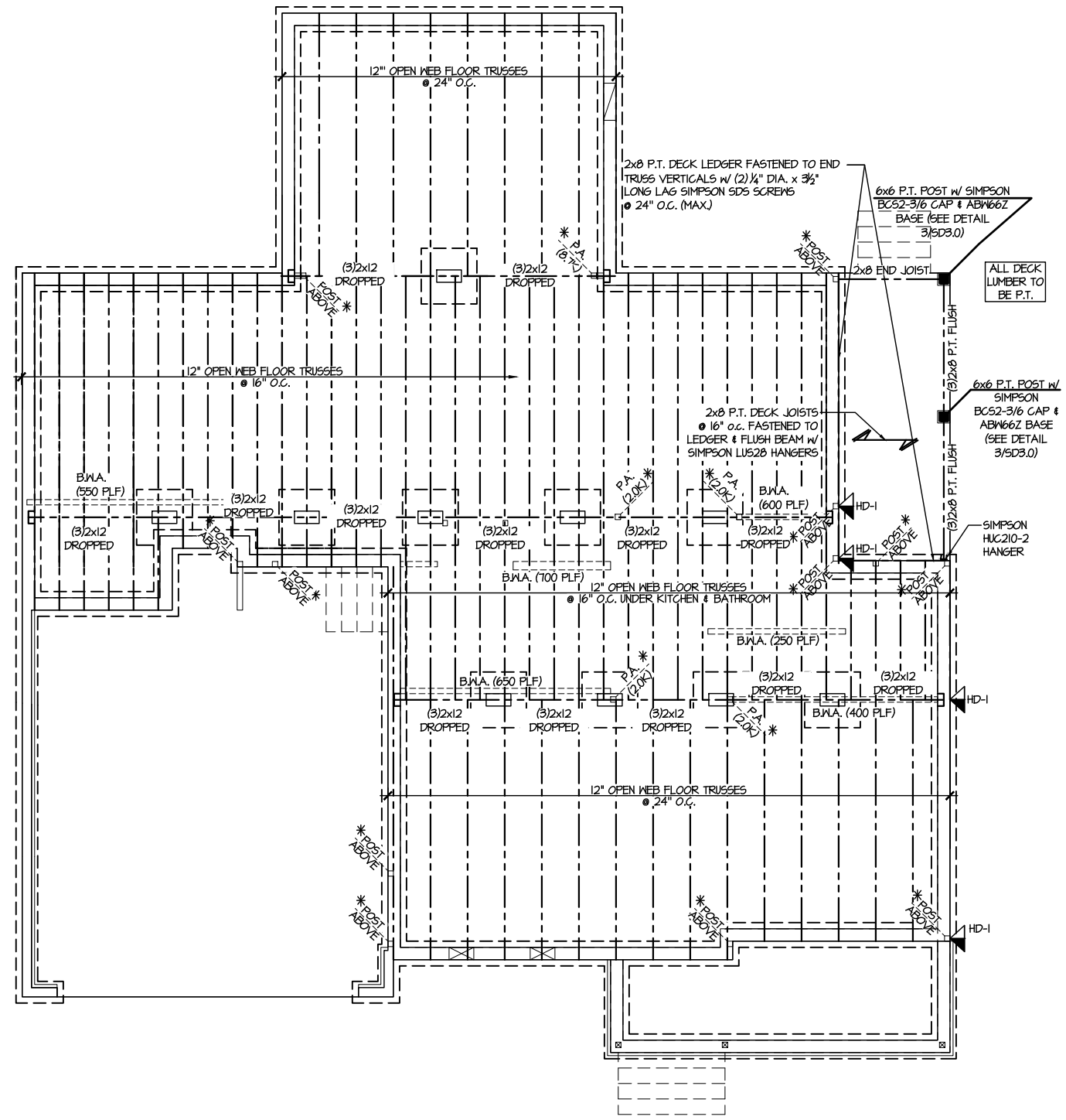
1 1ST FLOOR FRAMING PLAN (CRAWLSPACE) SCALE: 1/8"=1'-0"
