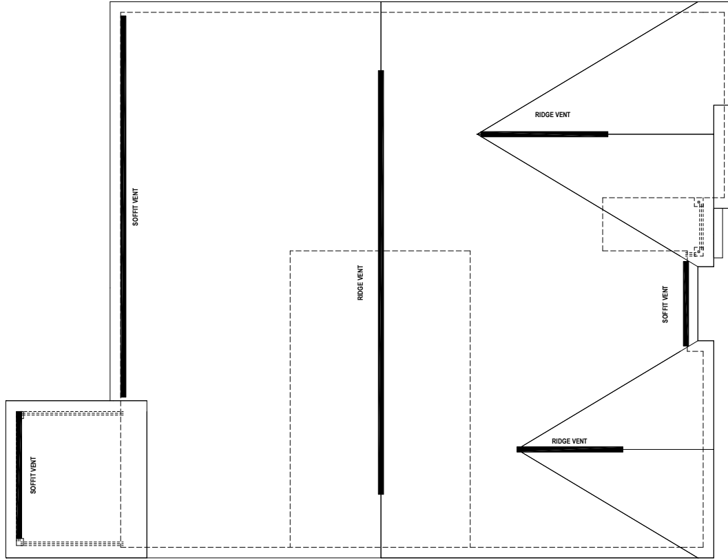
ROOF PLAN CALCS "A"
