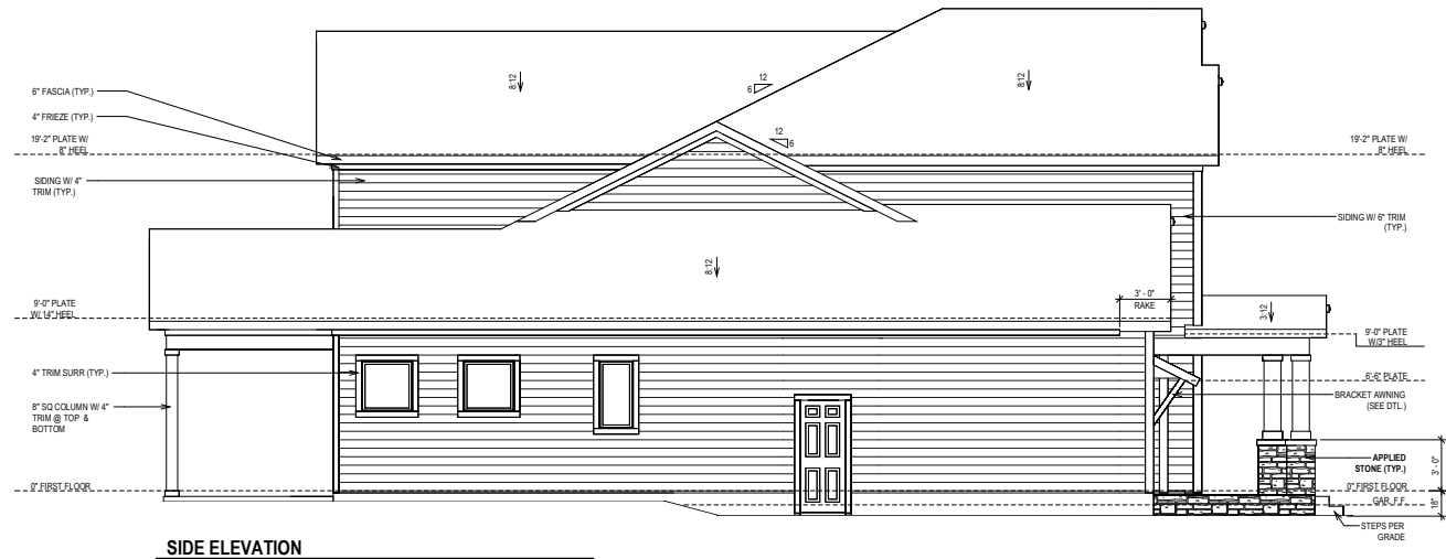
SIDE ELEVATION
