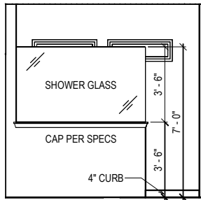
OWNER'S BATH
