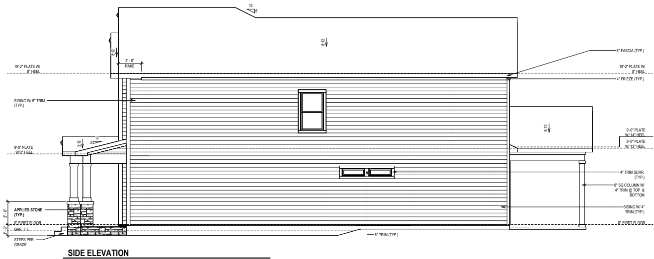
SIDE ELEVATION
