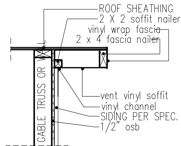
RAKE w/SIDING
